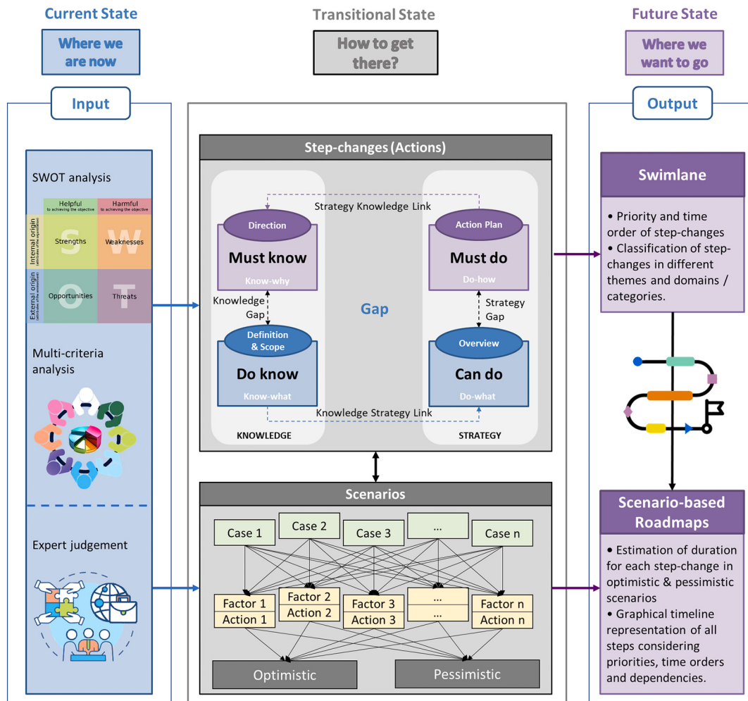
Fig. 1. Roadmapping framework.
