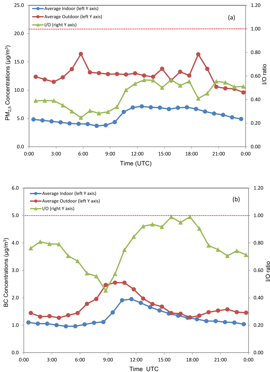
Fig. 4. Hourly average indoor and outdoor \text{PM}_{2.5} (a) and BC (b) concentrations in the maps file room.
