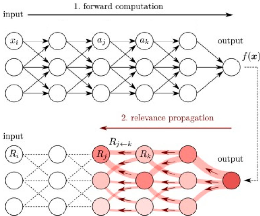
Fig. 2. Diagram of the LRP procedure (Montavon et al., 2018). Red arrows indicate the relevance propagation flow. (For interpretation of the references to colour in this figure legend, the reader is referred to the Web version of this article.) ( http://www.heatmapping.org/ .)
