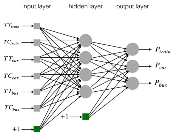
Fig. A2. Three-layers Artificial Neural Network.
