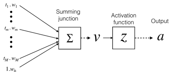
Fig. A1. A neuron layout.
