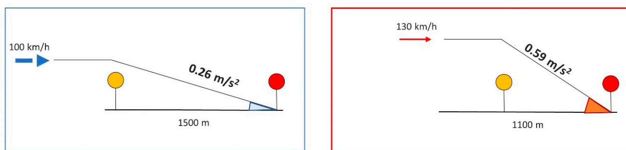
Figure 3. There is variation in the necessary rate of deceleration. In the left approach, a continuous deceleration rate of 0.26 \text{ m/s}^2 is sufficient to stop in front of the red signal, while the approach on the right requires a deceleration rate of at least 0.59 \text{ m/s}^2 .
