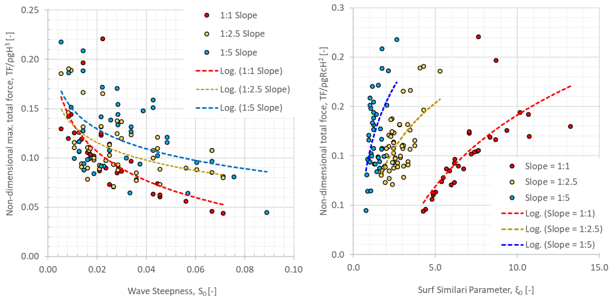
Fig. 11. Non-dimensional max non-dimensional total wave forces ( TF_{\max}^* = TF_{\max}/pgR_cH^2 )
