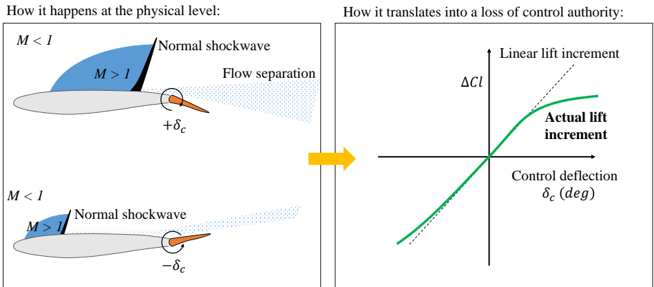
Figure 1.3: Illustration of the transonic shock position and its interaction with a control surface deflection.
