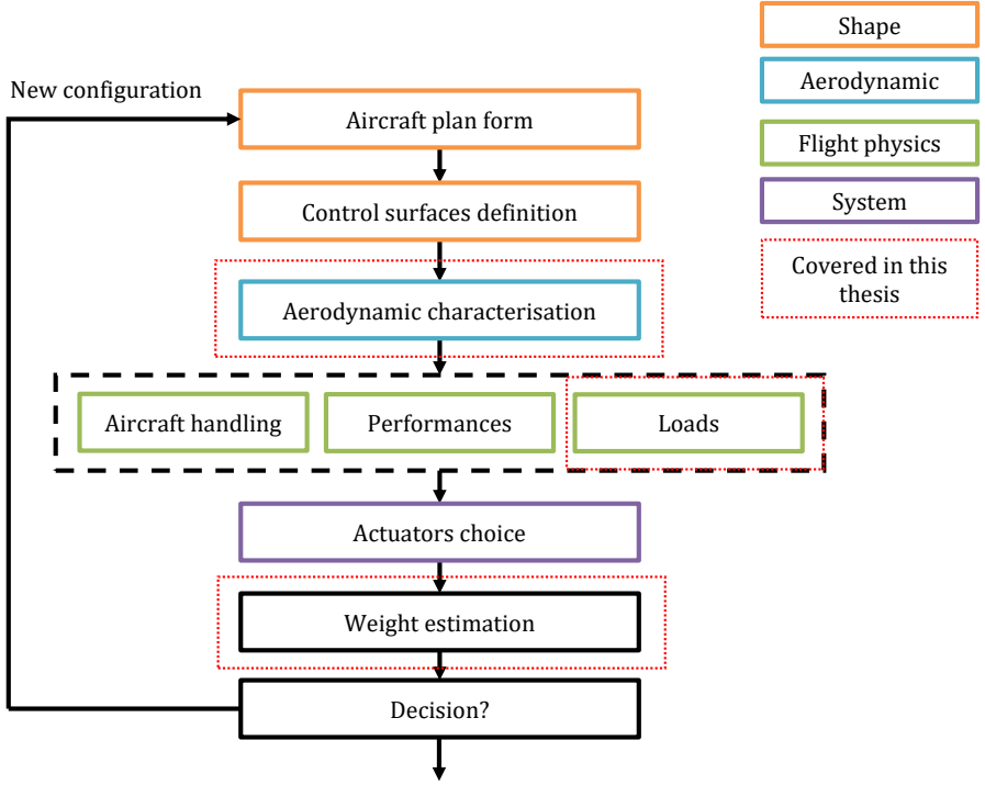
Figure 1.6: Industrial process for sizing control surfaces. Illustration adapted from Bertrand (2008).
