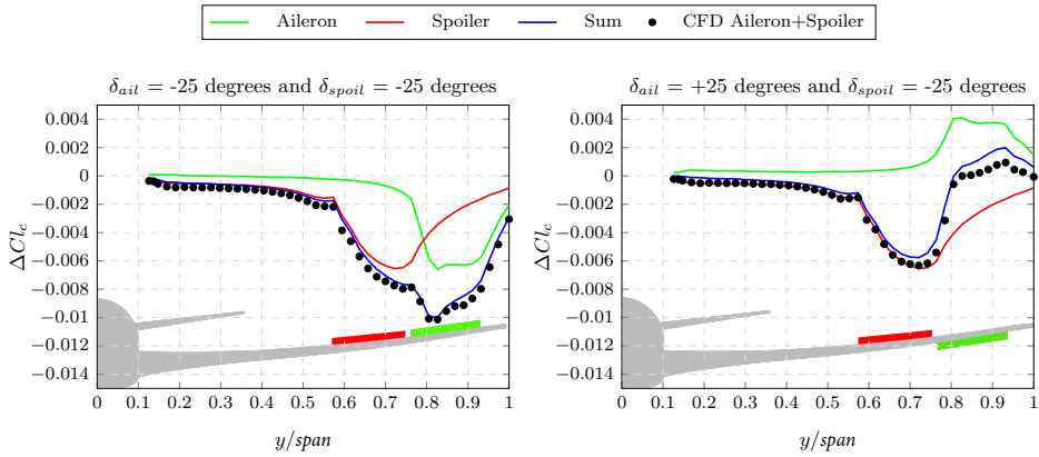
Figure 4.16: Rigid incremental lift distribution span-wise obtained with both the aileron and spoiler deployed.
