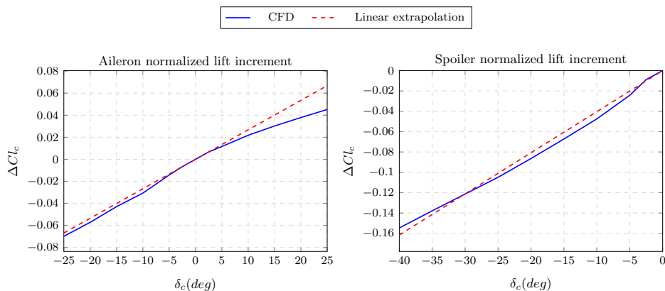
Figure 4.13: Lift increment obtained on the 3D wing for the aileron and the spoiler. The linear trends are interpolated around the 0 degrees position for the aileron, and with a least square fit for the spoiler.
