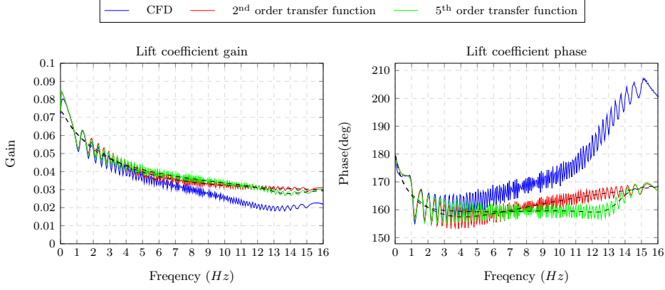
Figure 2.4: Frequency response plot of the CFD and transfer function results. The black dashed line indicates the exact response derive from the RFA polynomials.
