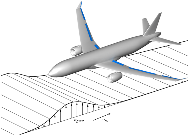
Figure 1.1: Illustration of a vertical gust hitting an aircraft in flight. Control surfaces (in blue) on the wings trailing edges and winglets can help reducing gust loads.
