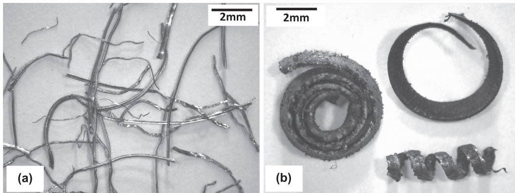
Fig. 1. Optical images of the metallic waste used: (a) steel wool fibres and (b) steel shavings.
