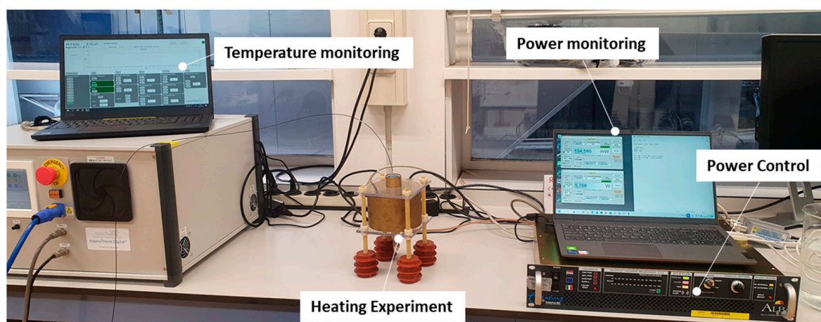
Figure 3. The experimental setup. Temperature monitoring is performed through a fiberoptic temperature sensor inserted in the PP vial. The applicator power is controlled through a 434 MHz power amplifier and monitored through power meters connected through a bidirectional coupler to the RF power output.
