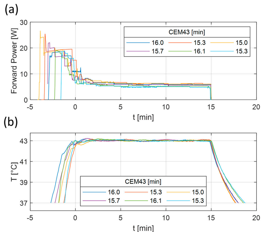
Figure 6. Measured forward power (a) and temperature (b) results of six repeated heating experiments. The heating experiments were planned to deliver 43 °C for 15 min. The lines correspond to the measured temperature distribution at the tip of the vial. The corresponding CEM43 values of each experiment are visible in the legend.
