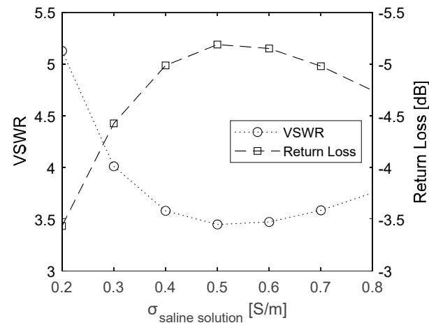
Figure 4. VSWR and Return Loss values calculated as a function of saline solution conductivity.
