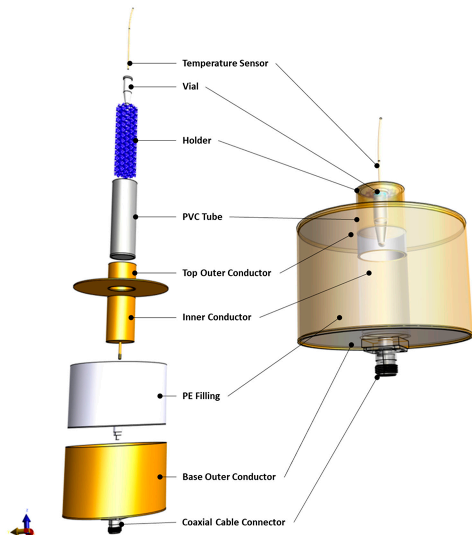
Figure 2. Model of the RF applicator components separately ( left ) as well as assembled ( right ).
