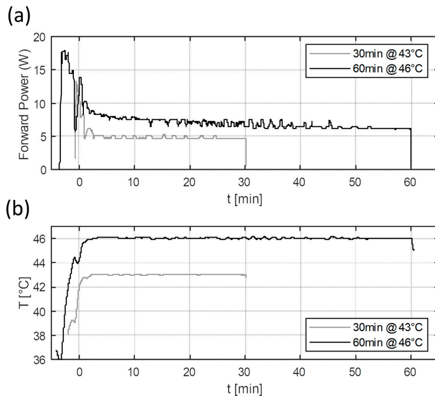
Figure 7. Measured forward power (a) and temperature (b) results of the two heating experiments. The heating experiments were planned to deliver 43 °C for 30 min and 46 °C for 60 min. The lines correspond to the measured temperature distribution at the tip of the vial.
