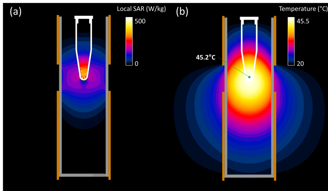
Figure 5. Simulated local SAR (a) and steady-state temperature (b) spatial distribution in the central cross-section of the RF applicator when applying 3 W of effective power. The temperature reached at the measuring point is indicated in the latter plot.
