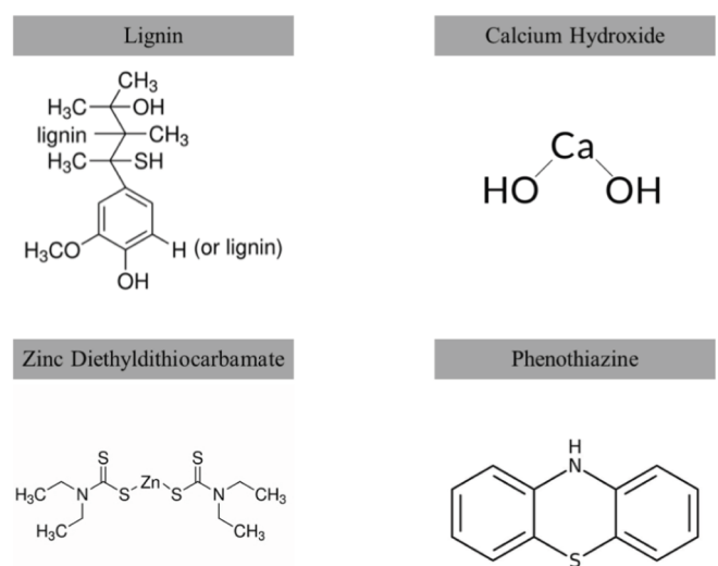
Fig. 1. Chemical structure of antioxidants used in the study.
