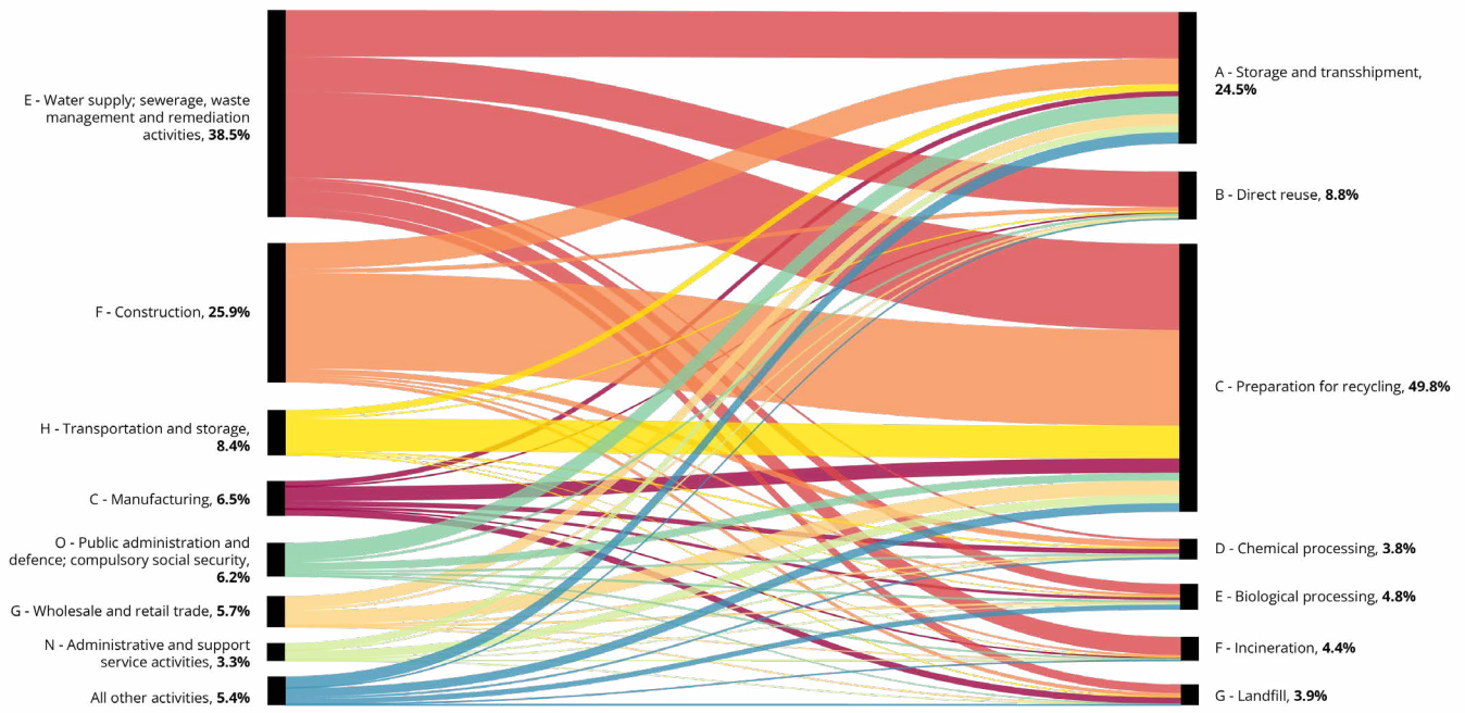
Figure 7.2. Waste distribution between economic sectors according to the NACE classification and the applied waste processing method. The distribution is based only on the high confidence matches.
