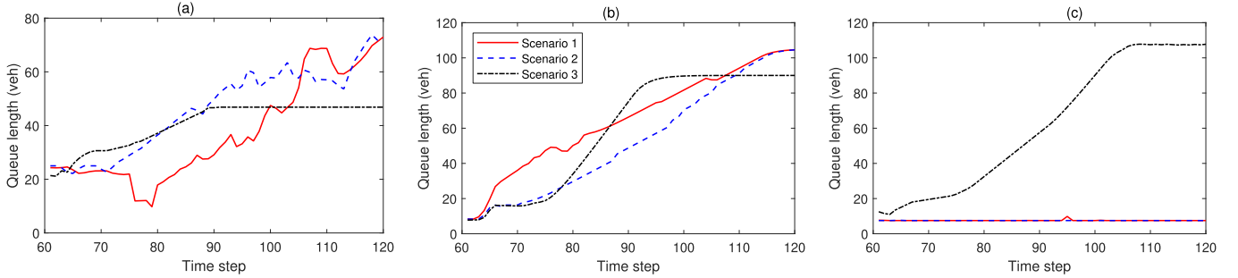
Fig. 13. Queue lengths of section 1, 2 and 3 in Fig. 11 in scenarios 1, 2, and 3. (a), (b), and (c) are queue lengths of destinations B, D, and F. Red, blue, and lines represent scenarios 1, 2, and 3 respectively.
