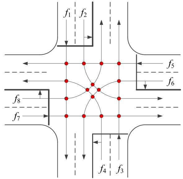
Fig. 3. An example intersection to explain the model variables. The figure is taken from [23]. f_1, f_2, \dots, f_8 are the flows of intersection links. Red dots in the figure represent conflicting points of flows. The intersection is indexed as intersection 1. For simplicity, we assume that there are four phases in a cycle, and W_1^1 = \{1, 3\} , W_1^2 = \{2, 4\} , W_1^3 = \{5, 7\} , W_1^4 = \{6, 8\} . Note that there can be more phases in a cycle as long as the movements in each cycle do not conflict. u_1^1, u_1^2, u_1^3 and u_1^4 are the green time fraction of each phase so the traffic light cycle constraint is: u_1^1 + u_1^2 + u_1^3 + u_1^4 \leq 1 . Green time fraction constraints are: f_1 \leq u_1^1 \cdot Q_1 , f_2 \leq u_1^2 \cdot Q_2 , f_3 \leq u_1^1 \cdot Q_3 , f_4 \leq u_1^2 \cdot Q_4 , f_5 \leq u_1^3 \cdot Q_5 , f_6 \leq u_1^4 \cdot Q_6 , f_7 \leq u_1^3 \cdot Q_7 , f_8 \leq u_1^4 \cdot Q_8 .
