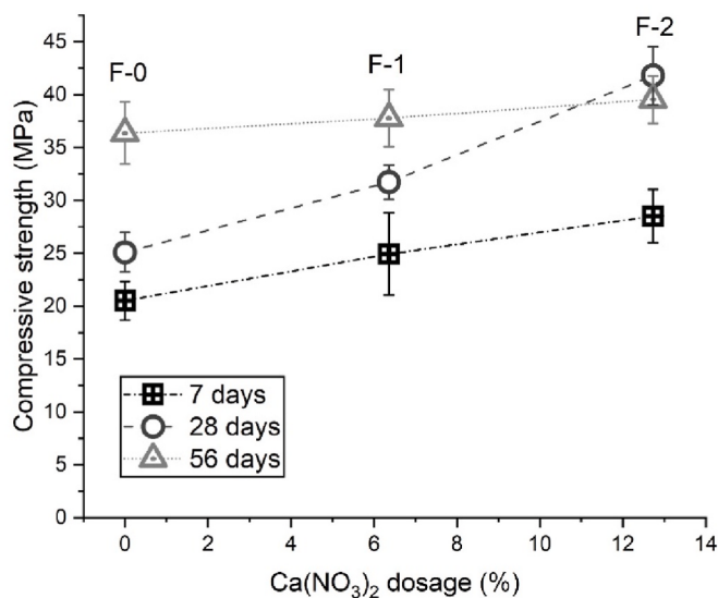
Fig. 14. Compressive strength of different studied mixtures at 7, 28 and 56 days. Error bars mean the standard deviation of repeated test results.
