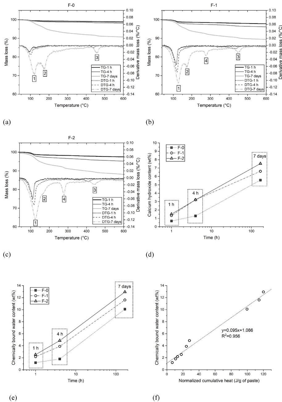
Fig. 12. TGA of different final mixtures at 1 h, 4 h, and 7 days: (a) TG and DTG curves of mixture F-0; (b) TG and DTG curves of mixture F-1; (c) TG and DTG curves of mixture F-2. 1- ettringite and C-S-H, 2- CO 3 -AFm, 3- calcium hydroxide (portlandite), 4- NO 3 -AFm. (d) Calcium hydroxide content normalized by the dry sample mass at 600 °C; (e) The content of chemically bound water normalized by the dry sample mass at 600 °C; (f) The correlation between normalized cumulative heat and chemically bound water content.
