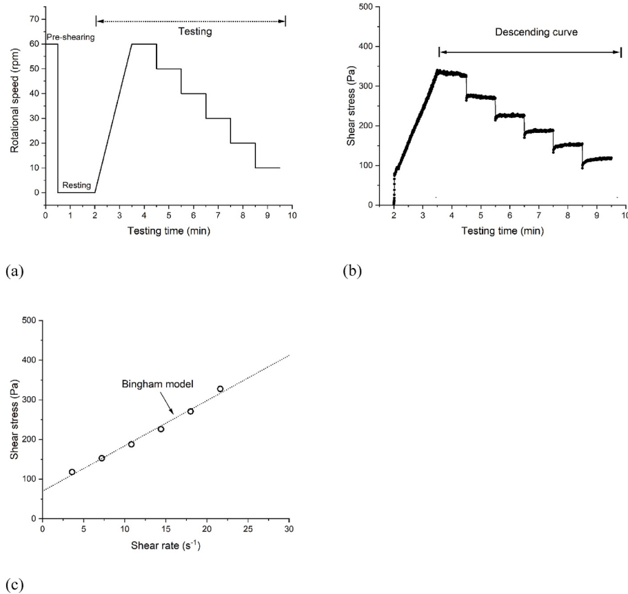
Fig. 4. Flow curve test: (a) Test protocol; (b) An example of shear stress and testing time curve; (c) The average shear stresses at the different shear rates (acquired from the descending curve) were plotted and fitted by the Bingham model.
