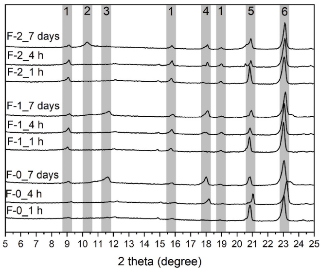
Fig. 13. XRD results of different final mixtures at 1 h, 4 h, and 7 days. 1- ettringite, 2- \text{NO}_3 -AFm, 3- \text{CO}_3 -AFm, 4- calcium hydroxide (portlandite), 5- quartz, 6- calcite.
