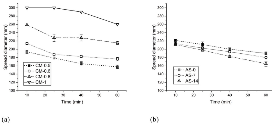
Fig. 5. Flowability test results: (a) Cementitious materials with different superplasticizer dosages – spread diameter at different resting times; (b) Acceleration slurries with different accelerator dosages – spread diameter at different resting times. Error bars mean the standard deviation of repeated test results.
