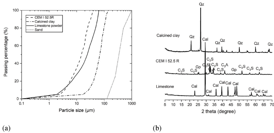
Fig. 3. (A) Particle size distribution of CEM I 52.5 R Portland cement, limestone and calcined clay determined by laser diffractometry. Quartz sand with grain size in the range of 0.125–1 mm; (b) X-ray diffraction patterns (Cu-K \alpha radiation) of CEM I 52.5 R Portland cement, calcined clay, and limestone powder. Qz - quartz, Gp - gypsum, Cal - calcite.
