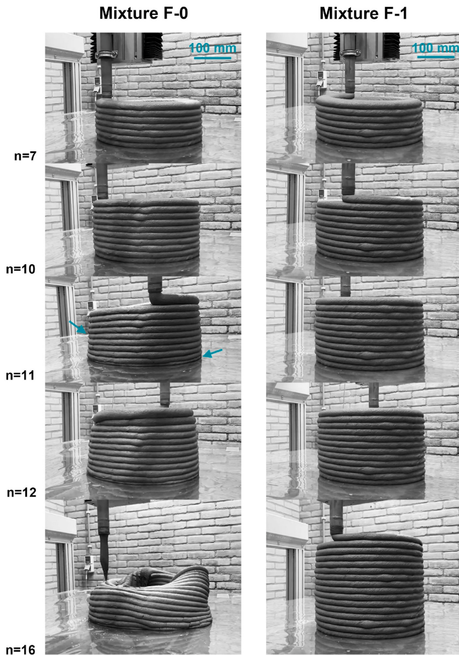
Fig. 10. Buildability test results (hollow cylinder with 250 mm printing path diameter) of mixtures F-0 and F-1. The cyan arrows indicated the onset of plastic deformation. (For interpretation of the references to colour in this figure legend, the reader is referred to the Web version of this article.)
