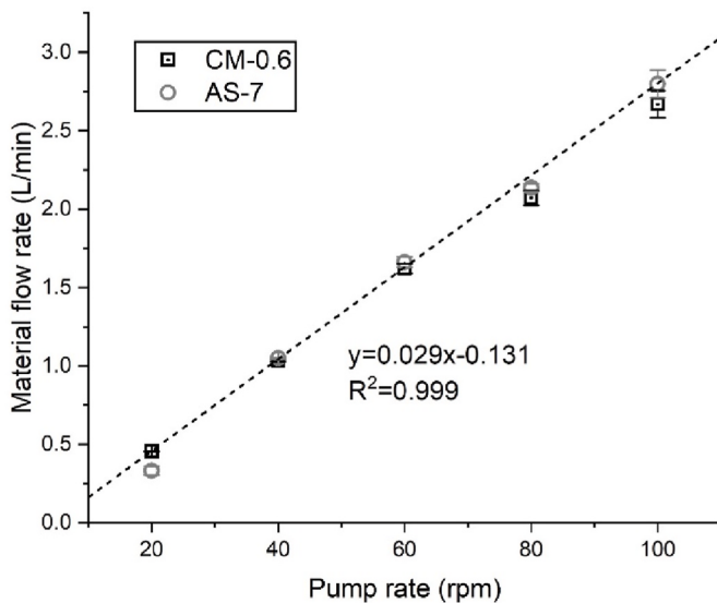
Fig. 7. Pumpability test results (material flow rates at the different pump rates) of mixtures CM-0.6 and AS-7. Error bars mean the standard deviation of repeated test results.
