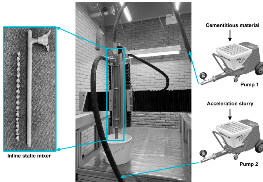
Fig. 1. Set-on-demand 3D concrete printing setup: CNC configuration, progressive-cavity pump ( \times 2 ), material hose ( \times 2 ), inline static mixer.
