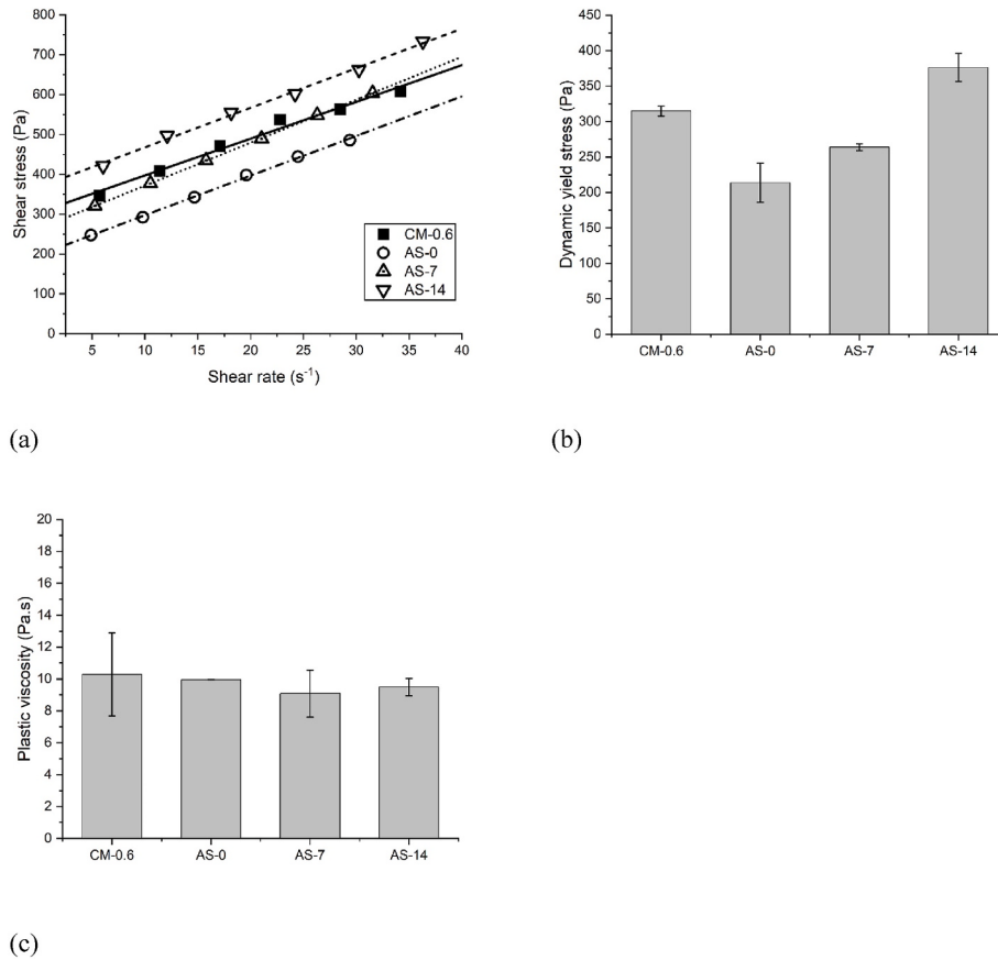
Fig. 6. Flow curve test results: (a) Shear stress as a function of shear rate (fitted by the Bingham model); (b) Dynamic yield stress and (c) plastic viscosity of different mixtures. Error bars mean the standard deviation of repeated test results.
