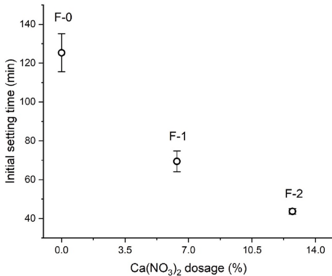
Fig. 8. Initial setting time results of final mixtures with different accelerator dosages. Error bars mean the standard deviation of repeated test results.
