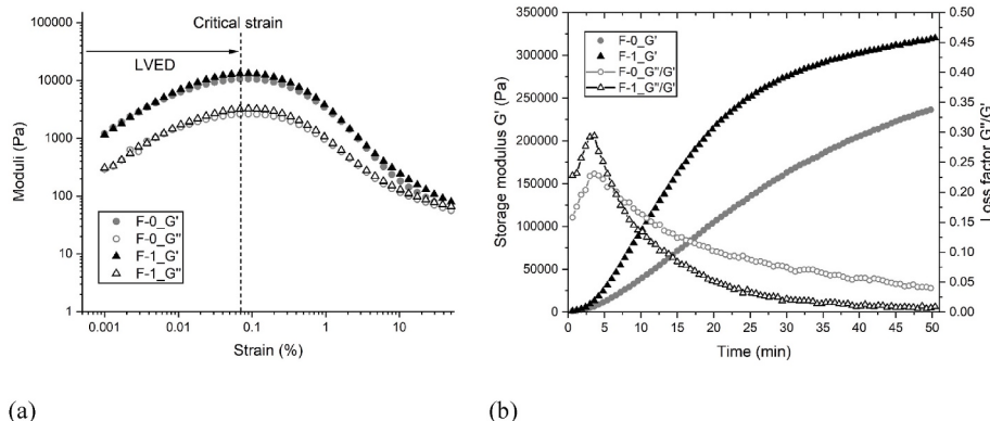
Fig. 9. SAOS test results: (a) Strain sweep of mixtures F-0 and F-1; (b) Time sweep of mixtures F-0 and F-1.
