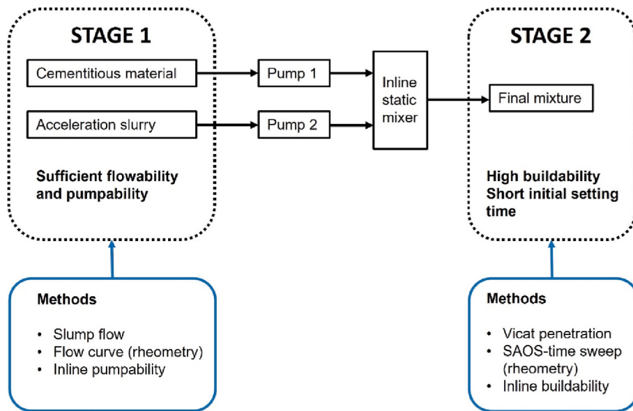
Fig. 2. A roadmap to develop set-on-demand limestone-calcined clay-based printable cementitious materials. Flowable and pumpable cementitious materials and acceleration slurries were formulated in stage 1, and the final mixture that displayed sufficient buildability was developed in stage 2.
