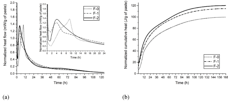
Fig. 11. Isothermal calorimetry test results: (a) Heat flow normalized by paste weight with time (24 h and 126 h); (b) Cumulative heat normalized by paste weight with time (7 days).
