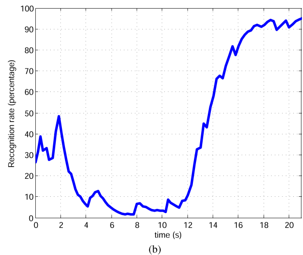
Fig. 8. Experimental results with “rice dream” box. (a) Snapshots from an experiment without occlusion. Initial view (left). Final view (right). (b) Recognition probability versus time. The recognition rate increases over time and hits 95%.
