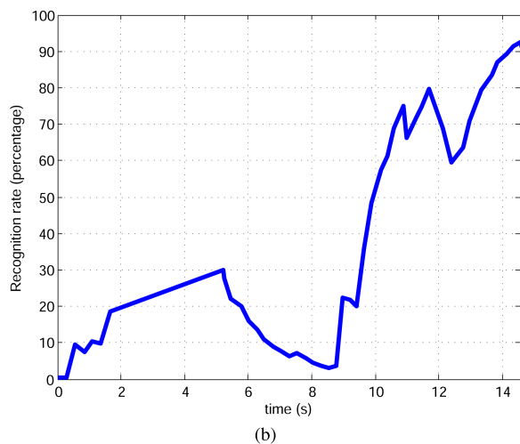
Fig. 7. Experimental results with “hagel slag” box. (a) Snapshots from an experiment without occlusion. Initial view (left). Final view (right). (b) Recognition probability versus time. The recognition rate increases over time and hits 95%.
