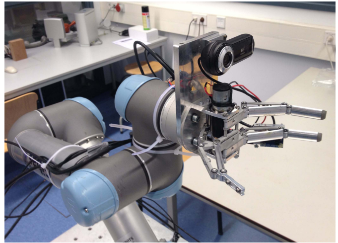
Fig. 11. Eye-in-hand system formed with a UR5 type universal robot arm, a Delft Hand 3 gripper, and a Logitech webcam.
