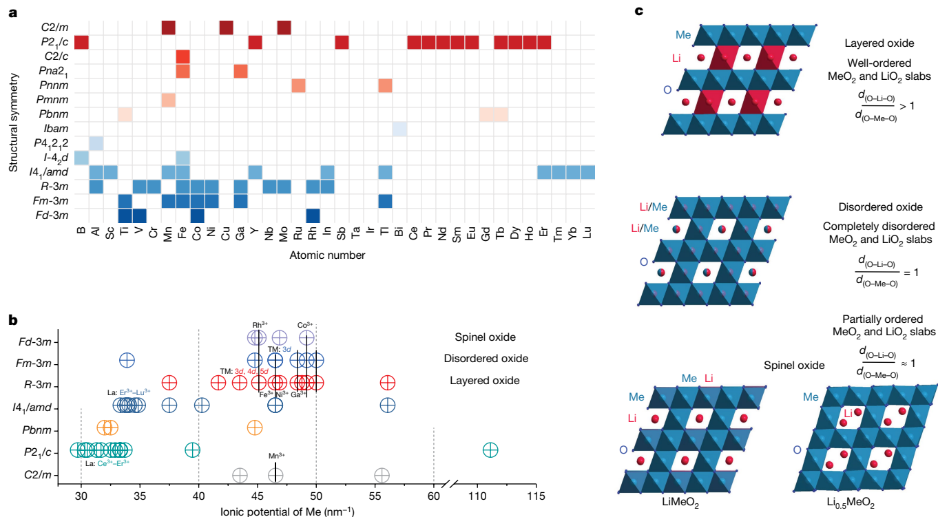
Fig. 1 | Screening the crystal structure of \text{LiMeO}_2 compositions. a , Structural symmetry of \text{LiMeO}_2 compositions. Me is the trivalent metal ion (Supplementary Figs. 1–14 and Supplementary Tables 1 and 2). b , Ionic potential of Me ions in \text{LiMeO}_2 compositions. c , Structure transformation in layered, disordered and spinel oxides, and their corresponding d_{(\text{O-Li-O})}/d_{(\text{O-Me-O})} , where d_{(\text{O-Li-O})} is
