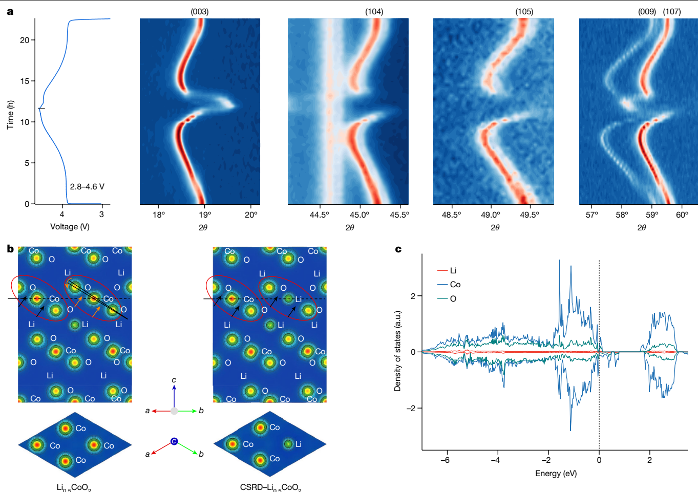
Fig. 4 | Crystal and electronic structure information of the CSRD-LiCoO 2 cathode. a , In situ XRD patterns recorded at a current rate of 0.08 C in the voltage range of 2.8–4.6 V. b , Charge density distribution of the CSRD-LiCoO 2 and the regular LiCoO 2 cathodes after the de-lithiation to Li 0.5 CoO 2 . The red
