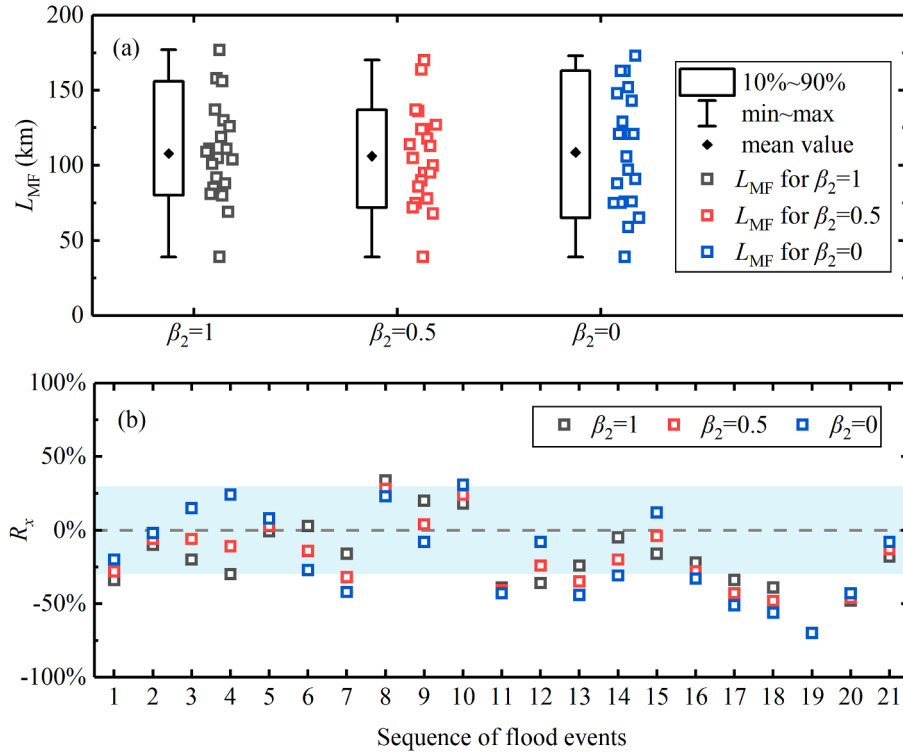
Fig. 5. (a) Boxplot of the calculated value of L_{MF} (the calculated values are shown to the side as gray, red, and blue dots which correspond to the value of L_{MF} with \beta_2 taking 1, 0.5, and 0, respectively), and (b) relative deviation of the L_{MF} from the L_{XH} . The blue shaded area indicates the interval with deviation less than 30 %, i.e., |R_x| < 30 \% .
