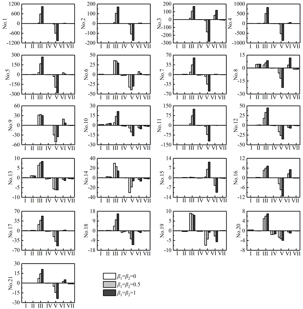
Fig. 11. Estimated values of each influencing term normalized by the discharge increment for strategy 2.
