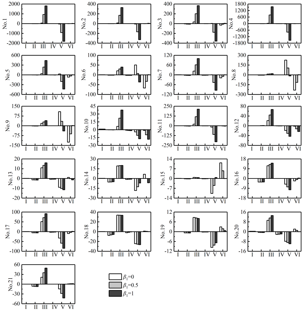
Fig. 10. Estimated values of each influencing term normalized by the discharge increment for strategy 1.
