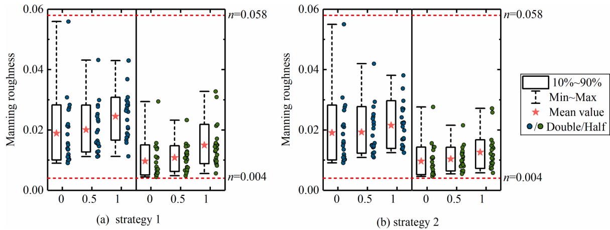
Fig. 16. The range of Manning roughness corresponds to the variation of bed slope in (a) strategy 1 and (b) strategy 2.
