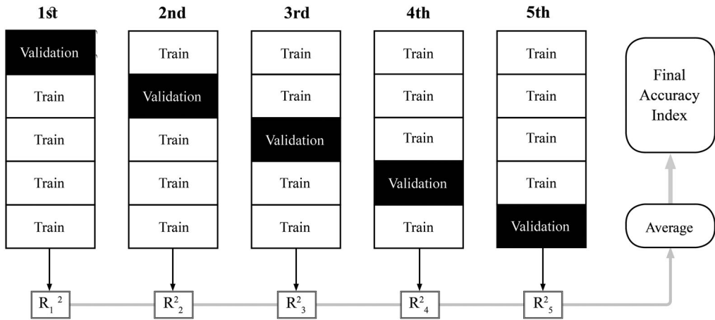
Figure 5. Cross-validation.
