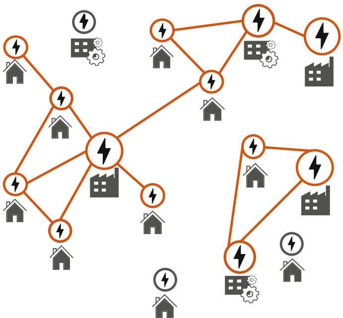
Fig. 2.4 Distributed energy system. Source designed by the Authors
