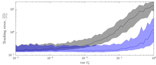
(b) Varying noise level \text{var}(e_k) , and p = f = 20 with \bar{N} = 200 .
