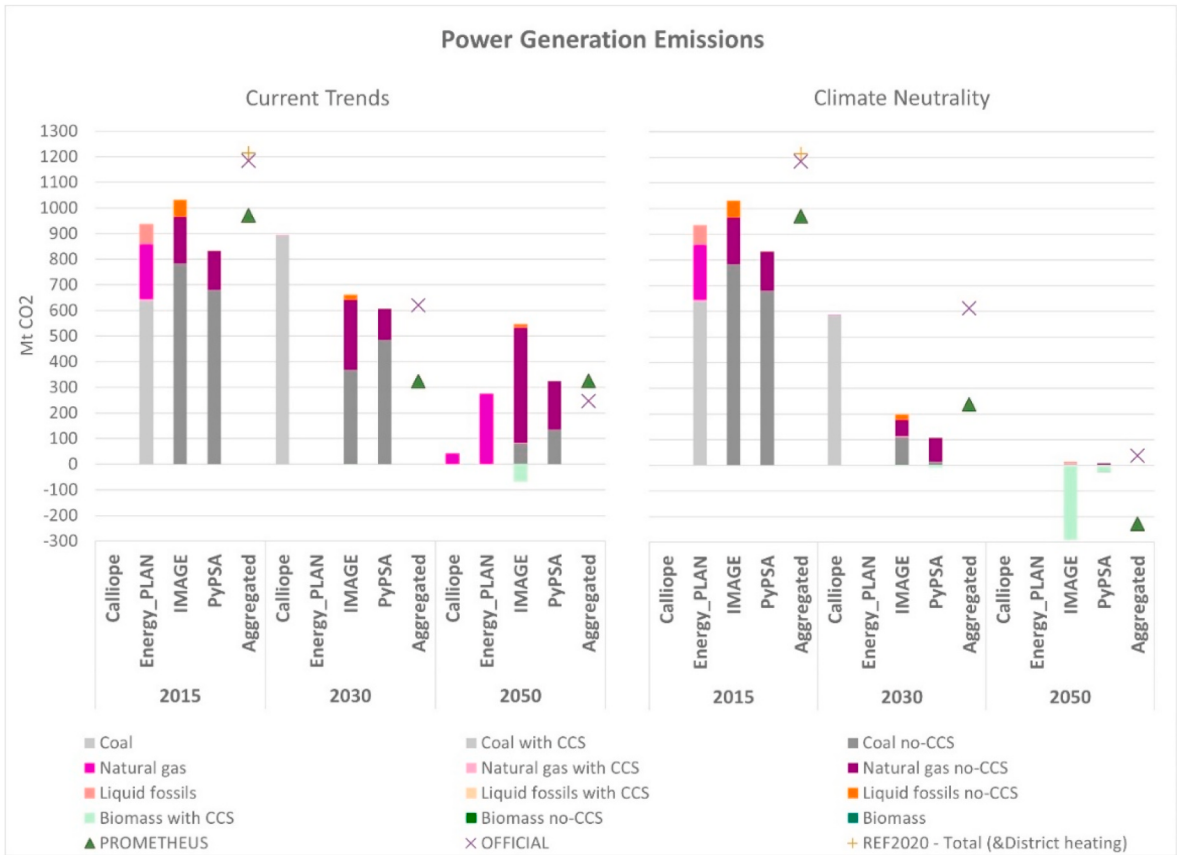
Fig. B3. CO 2 emissions from electricity generation for the Europe region under Current Trends and Climate Neutrality scenarios. The official EU scenario contains data from ‘A Clean Planet for all’ and ‘2030 Climate Target Plan’ (European Commission, 2018b, 2020b). “External” category refers to data from the official EU scenario and the REF2020 scenario. Some models distinguish between carriers that are coupled with CCS and carriers that are not coupled to CCS.
