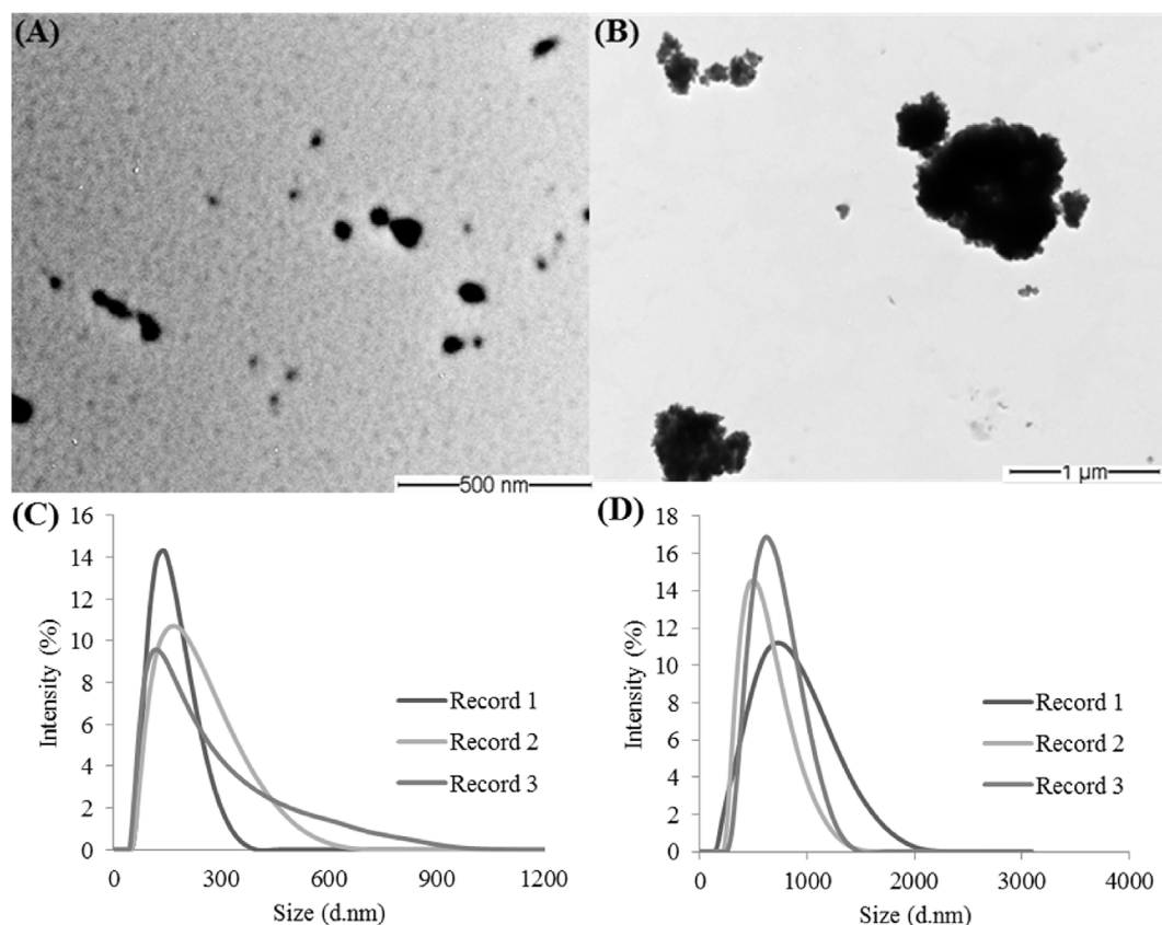
Fig. 1. Characteristics of (suspensions of) TiO 2 NPs. (A) TEM of TiO 2 NPs dispersed in milli-Q water. (B) TEM picture of TiO 2 NPs dispersed in soil extract. (C) Size distribution of TiO 2 NPs dispersed in milli-Q water. (D) Size distribution of TiO 2 NPs dispersed in soil extract.
