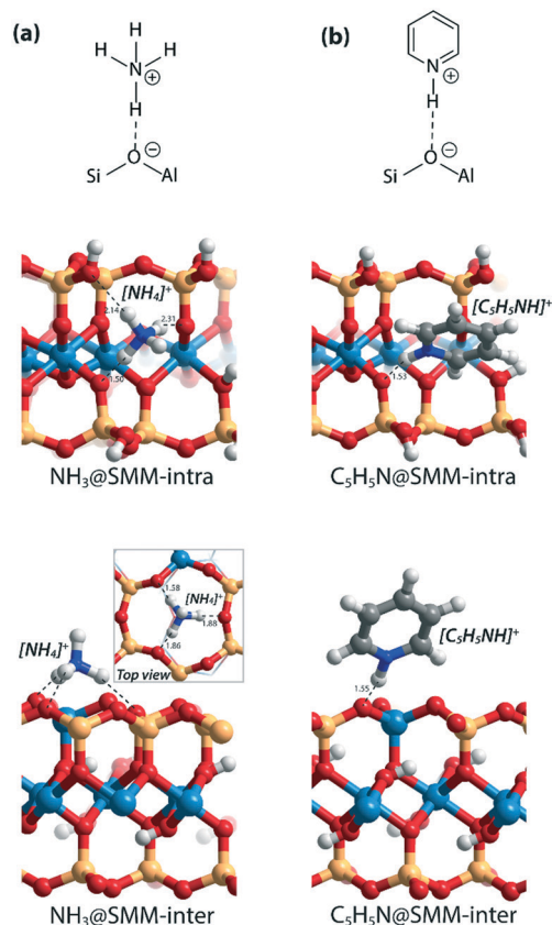
Fig. 3 Optimized structures of the adsorption complexes of (a) ammonia (NH 3 ) and (b) pyridine (C 5 H 5 N) in SMM-intra and SMM-inter models. Bond distances ( d ) are in Å.
