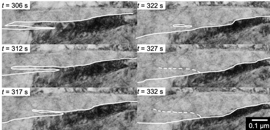
Figure 5.8. Formation of a new plate of bainite (lower plate) and its sideways merging with a preexisting plate of bainite. The upper plate of bainite is the plate shown in Figure 5.6b . The continuous white line marks the B/A interface, and the dotted white line marks the trace of where both plates merged. All times are relative to the time at which the image in Figure 5.6a 1 was taken. The images without the lines and annotations are shown in Figure C.2
