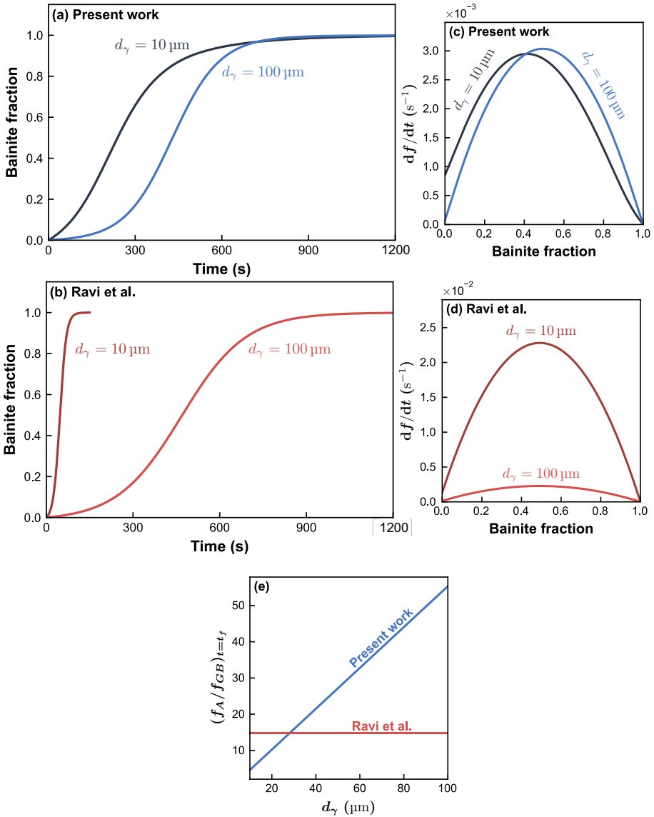
Figure 2.4. Effect of the prior austenite grain size on bainite formation according to the present model and Ravi et al. 's model. In all cases T = 300 \text{ }^\circ\text{C} and X_b = \bar{X} were considered. For the simulations using the model from the present work, Q_{AGB\bar{X}} = 200 \text{ kJ mol}^{-1} , Q_{BA\bar{X}} = 195 \text{ kJ mol}^{-1} , and u_T = 0.100 \mu\text{m} were used. In the simulations using Ravi et al. 's model, Q_{AGB\bar{X}} = 145 \text{ kJ mol}^{-1} , Q_{BA\bar{X}} = 125 \text{ kJ mol}^{-1} , T_h = 577 \text{ }^\circ\text{C} , and \alpha_m = 0.011 \text{ K}^{-1} were used. a-d. Simulated bainite fraction as a function of time and the rate of bainite formation as a function of bainite fraction for both models and for d_\gamma = 10 \mu\text{m} and d_\gamma = 100 \mu\text{m} . e. Ratio between the fraction of autocatalytic nucleated and grain boundary nucleated bainite at the end of the transformation as a function of prior austenite grain size for both models.
