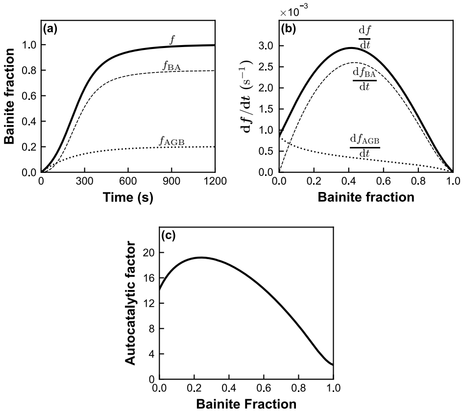
Figure 2.2. Simulated kinetics of bainite formation considering the parameters: T = 300^\circ\text{C} , d_\gamma = 10\ \mu\text{m} , Q_{AGB\bar{X}} = 200\ \text{kJ mol}^{-1} , Q_{BA\bar{X}} = 195\ \text{kJ mol}^{-1} , u_T = 0.100\ \mu\text{m} , and X_b = \bar{X} . a. Fraction of bainite over time, distinguishing the total fraction, f , the fraction nucleated by autocatalysis, f_{BA} , and the fraction nucleated at austenite grain boundaries, f_{AGB} . b. Rate of bainite formation, also showing the total rate and distinguishing individual components by nucleation site. c. Autocatalytic factor calculated by Equation (2.23)
