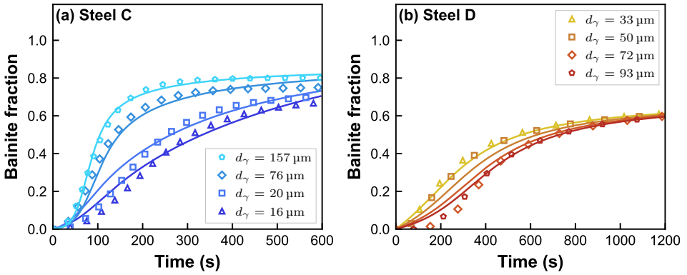
Figure 2.6. Experimental data (markers) and modeled curve (solid line) of bainite formation for a. steel C and b. steel D at different prior austenite grain sizes, alongside the best fit values for the initial activation energies. Since the retained austenite fraction for Steel D was not reported, it was estimated using the steel models from Thermo-Calc version 2023a with the thermodynamic database TCFE12 [37].
