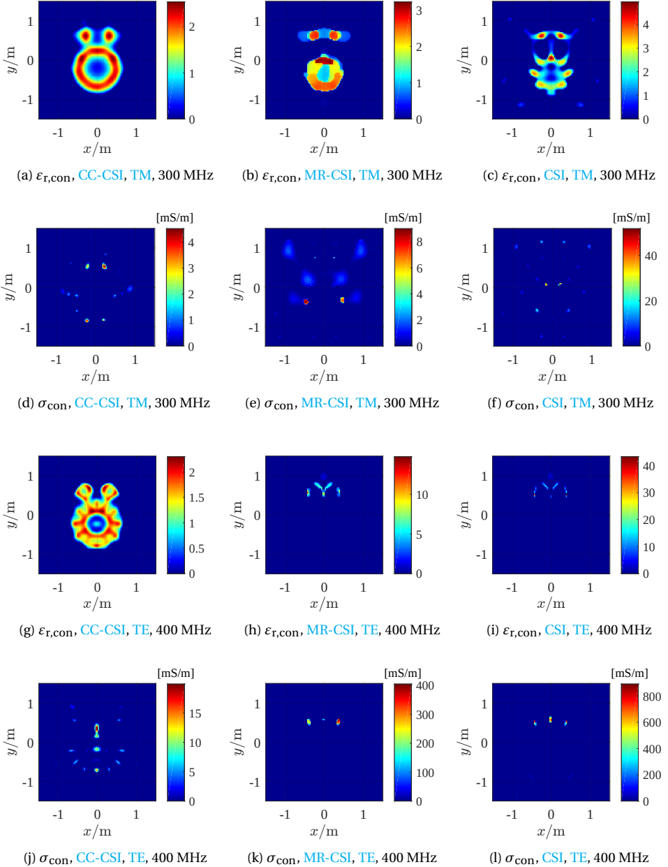
Figure 3.14: Reconstructed relative permittivity, \epsilon_{r,\text{con}} , and conductivity, \sigma_{\text{con}} , in Example 2 with 2048 iterations. SNR=30dB. (a-f) correspond to Fig. 3.13 (a); (g-l) correspond to Fig. 3.13 (d).
