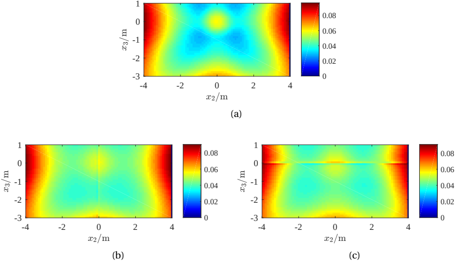
Figure 2.9: Computation error of the three components of the electric field on the cross section of x_1 = -0.1 . (a) E_{x_1} ; (b) E_{x_2} ; (c) E_{x_3} .
