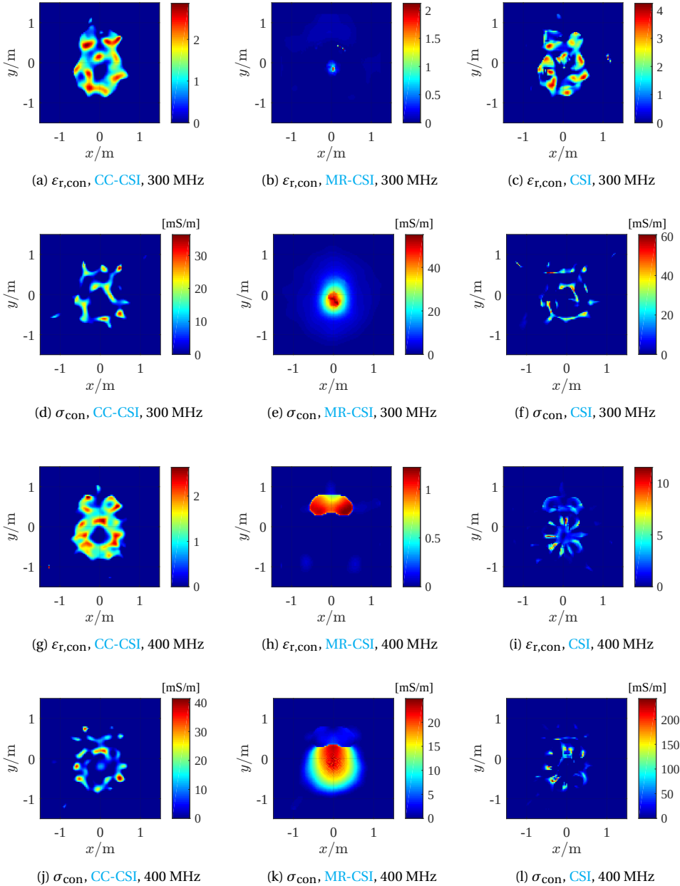
Figure 3.11: Reconstructed relative permittivity, \varepsilon_{r,\text{con}} , and conductivity, \sigma_{\text{con}} , in Example 1 with 2048 iterations. SNR= 10dB. TE -polarization data.
