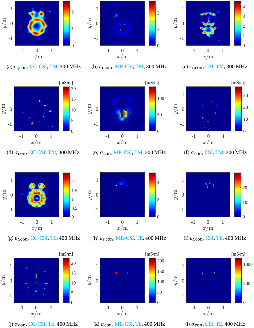
Figure 3.15: Reconstructed relative permittivity, \epsilon_{r,\text{con}} , and conductivity, \sigma_{\text{con}} , in Example 2 with 2048 iterations. SNR=10dB. (a-f) correspond to Fig. 3.13 (a); (g-l) correspond to Fig. 3.13 (d).
