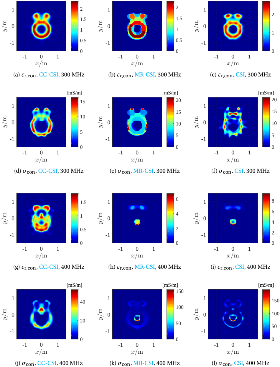
Figure 3.5: Reconstructed relative permittivity, \varepsilon_{r,\text{con}} , and conductivity, \sigma_{\text{con}} , in Example 1 with 2048 iterations. SNR=30dB. TM-polarization data.
