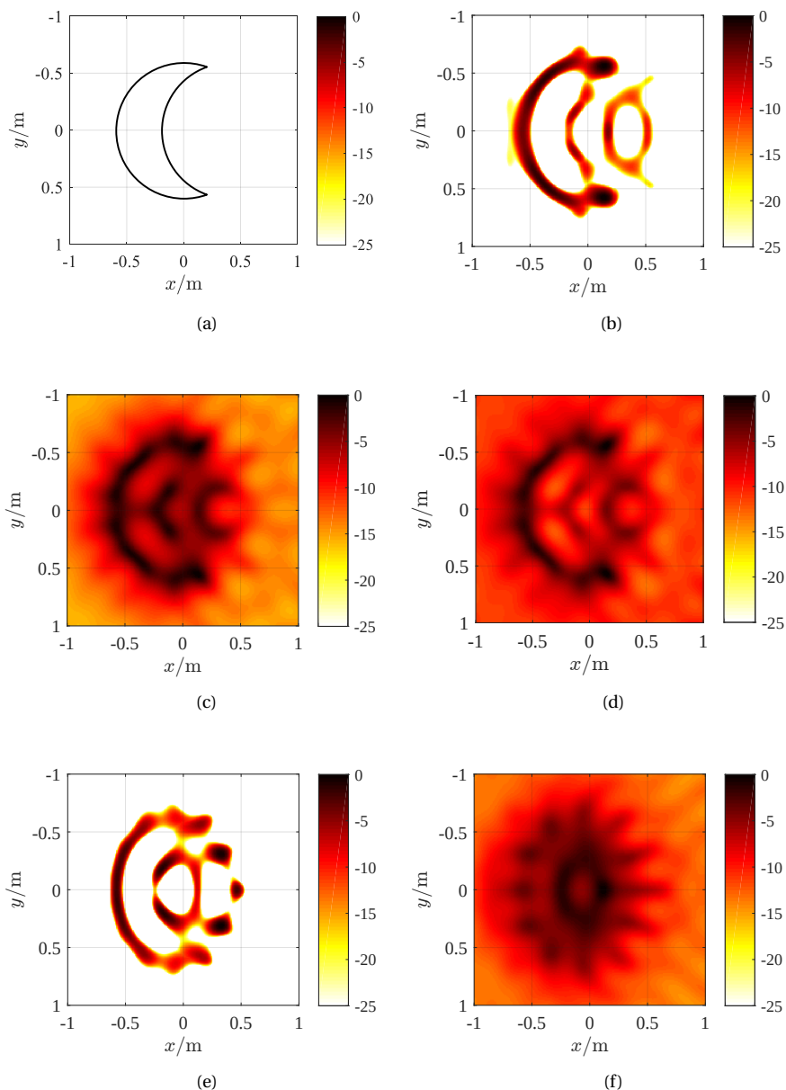
Figure 4.5: Scatterer geometry and its reconstructed shapes in Simulation 2. (a) Scatterer geometry; Reconstructed shape by processing the TM-polarized data with MMV (b), LSM (c), and the improved LSM with I = 6 (d), respectively. Reconstructed shape by processing the TE-polarized data with MMV (e) and LSM (f), respectively.
