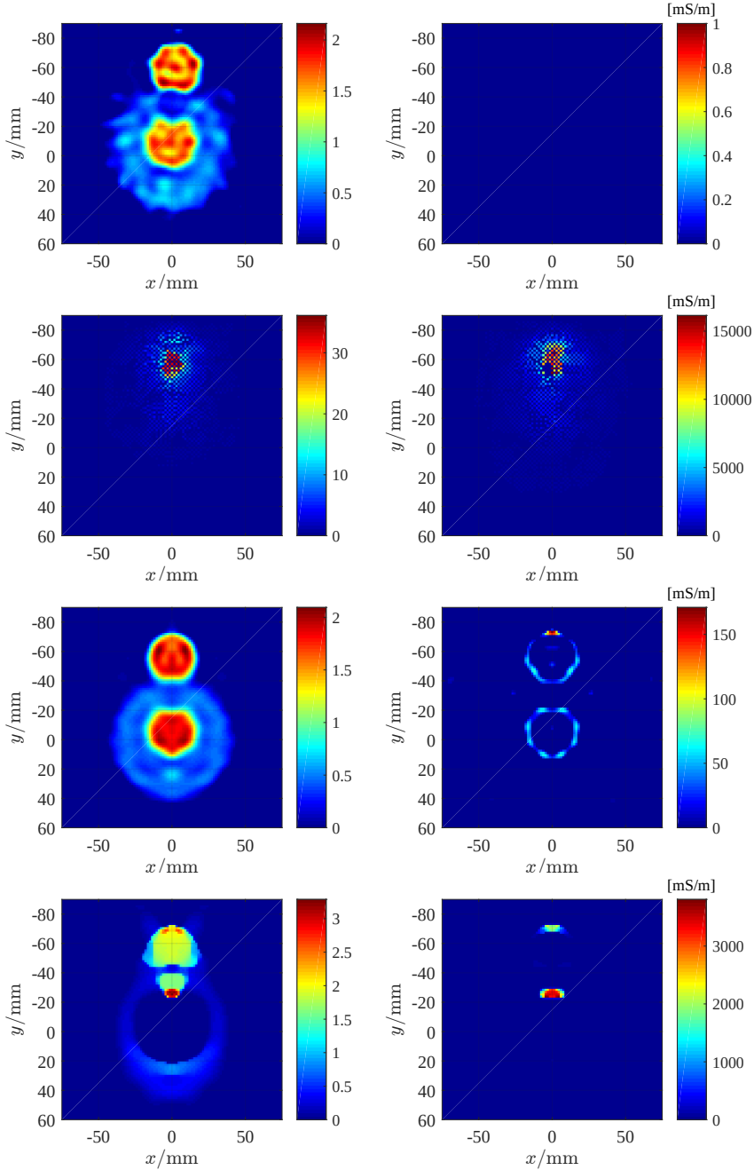
Figure 3.18: Relative permittivity (left) and conductivity (right) of the inverted contrast by processing the multi-frequency dataset FoamTwinDielTM (Line 1: MF-CC-CSI; Line 2: MF-MR-CSI) and its perfect synthetic data (Line 3: MF-CC-CSI; Line 4: MF-MR-CSI) at 7 GHz, 8 GHz, 9 GHz, and 10 GHz with 2048 iterations.
