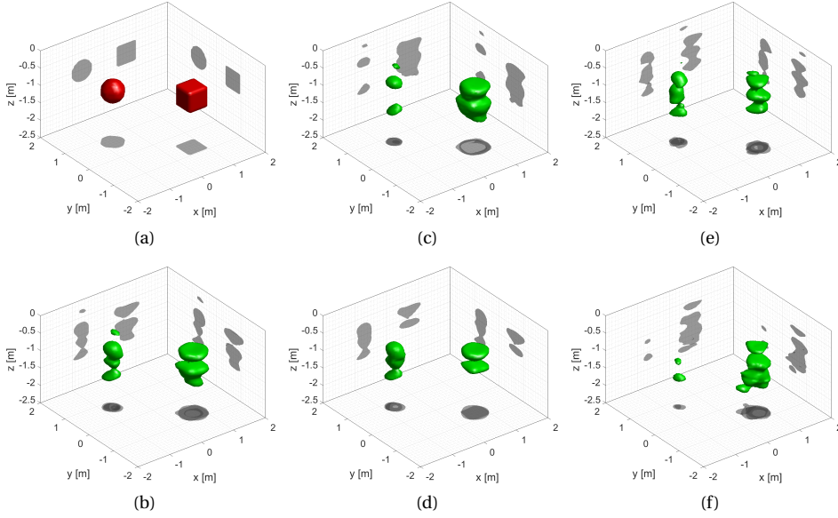
Figure 5.4: 3-D shape of the reconstructed results in the GPR imaging experiment at 200 MHz. 5% random white noise is added. (a): True objects. (b): Reconstructed contrast sources. Reconstructed contrast permittivity (c) and contrast conductivity (d) using the exact background model. Reconstructed contrast permittivity (e) and contrast conductivity (f) using an inexact background model ( 1.25\epsilon_{bg} ).
