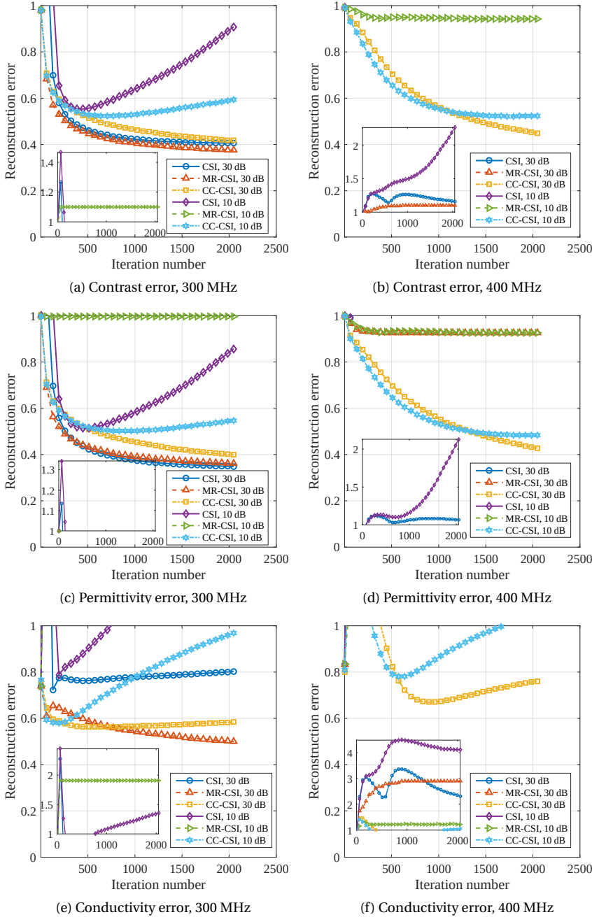
Figure 3.9: Reconstruction error curves of classical CSI, MR-CSI, and CC-CSI in the TE case of Example 1. Left: 300 MHz; Right: 400 MHz. (a), (b): complex contrast error, err_{\chi} ; (c), (d): permittivity error, err_{\epsilon} ; (e), (f): conductivity error, err_{\sigma} ;
