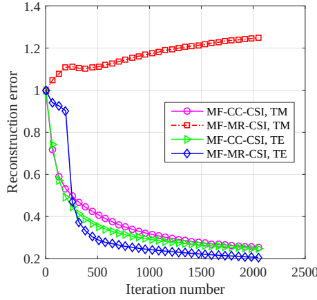
Figure 3.20: Inversion error curves of MF-CC-CSI and MF-MR-CSI in terms of iteration number in processing the multi-frequency perfect synthetic data of the Fresnel datasets, FoamTwinDielTM and FoamTwinDielTE , at 7 GHz, 8 GHz, 9 GHz, and 10 GHz.
