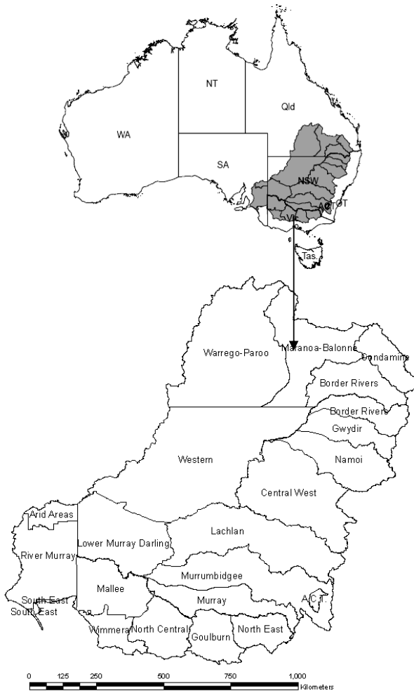
Figure 3: Case study area (Murray-Darling Basin Authority (MDBA)).
