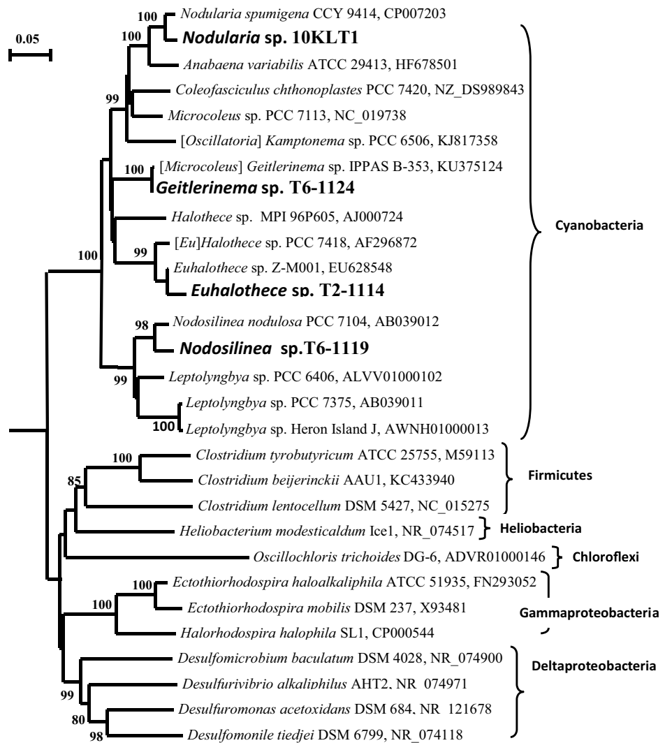
Fig. 4 16S rRNA gene-based phylogenetic tree showing the position of the studied new strains isolated from the Kulunda steppe soda lakes (marked in bold) among cyanobacteria. The tree was constructed with the use of the neighbor-joining algorithm. Scale bar shows evolutionary distance corresponding to 5 substitutions per 100 nucleotides. Numerals at the nodes show the statistical significance of the branching order as determined by bootstrap analysis of 1000 alternative trees (only values higher than 80% are shown). The cyanobacterial culture Nodularia sp. 10KLT1 was isolated from Tanatar 1 lake, Geitlerinema sp. T6-1124, Nodosilinea sp. T6-1119, and Euhalothece sp. T2-1114 which were isolated from Tanatar 2 and Tanatar 6 soda lakes
