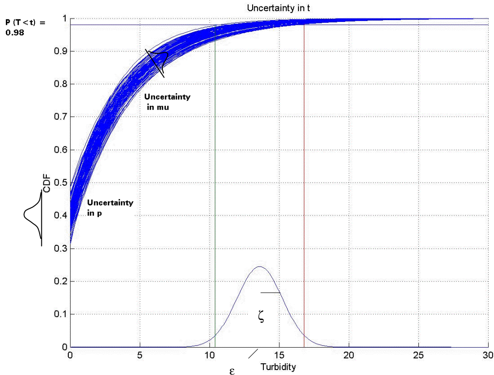
Figure 0-24 Cumulative Distribution Function of a B-E distribution with parameters p=0.4 and \mu=4 . The parameter uncertainties and the required reliability of 98% determine the allowable turbidity. In this figure 100 measurements were included. With more measurements the curve of the distribution of becomes more narrow and higher and the interval becomes smaller. This also happens for a lower reliability percentage but the curve will move to the left as well.
