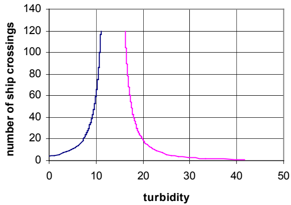
Figure 0-25 The interval of the allowable level of turbidity decreases with increasing number of ship crossings. p=0.4 , \mu=4
