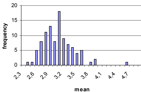
Figure 0-21 The distribution function of mean values, derived from a simulation of the BE distribution function with \mu = 3 and p = 0,1 can be modelled by a normal
