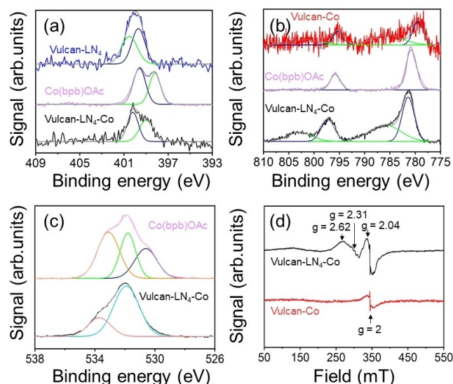
Figure 2. (a) N 1s XPS spectra of Vulcan-LN 4 , Vulcan-LN 4 -Co and Co(bpb)OAc, (b) Co 2p XPS spectra of Vulcan-LN 4 -Co, Vulcan-Co, and Co(bpb)OAc, (c) O 1s XPS spectra of Vulcan-LN 4 -Co and Co(bpb)OAc and (d) EPR spectra of Vulcan-Co and Vulcan-LN 4 -Co.
