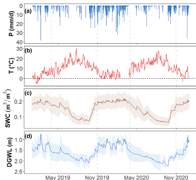
FIGURE 2 Time series of daily total precipitation amount (P) (mm/d) (a), daily average air temperature (T) (°C) (b), daily average soil water content (SWC) (m 3 /m 3 ) (c) and daily average depth to groundwater level (DGWL) (m) (d). The shaded bands in panels c and d represent the standard deviation from the mean of all monitoring sites. The vertical dashed lines delineate the two growing seasons (1 April to 31 October).
