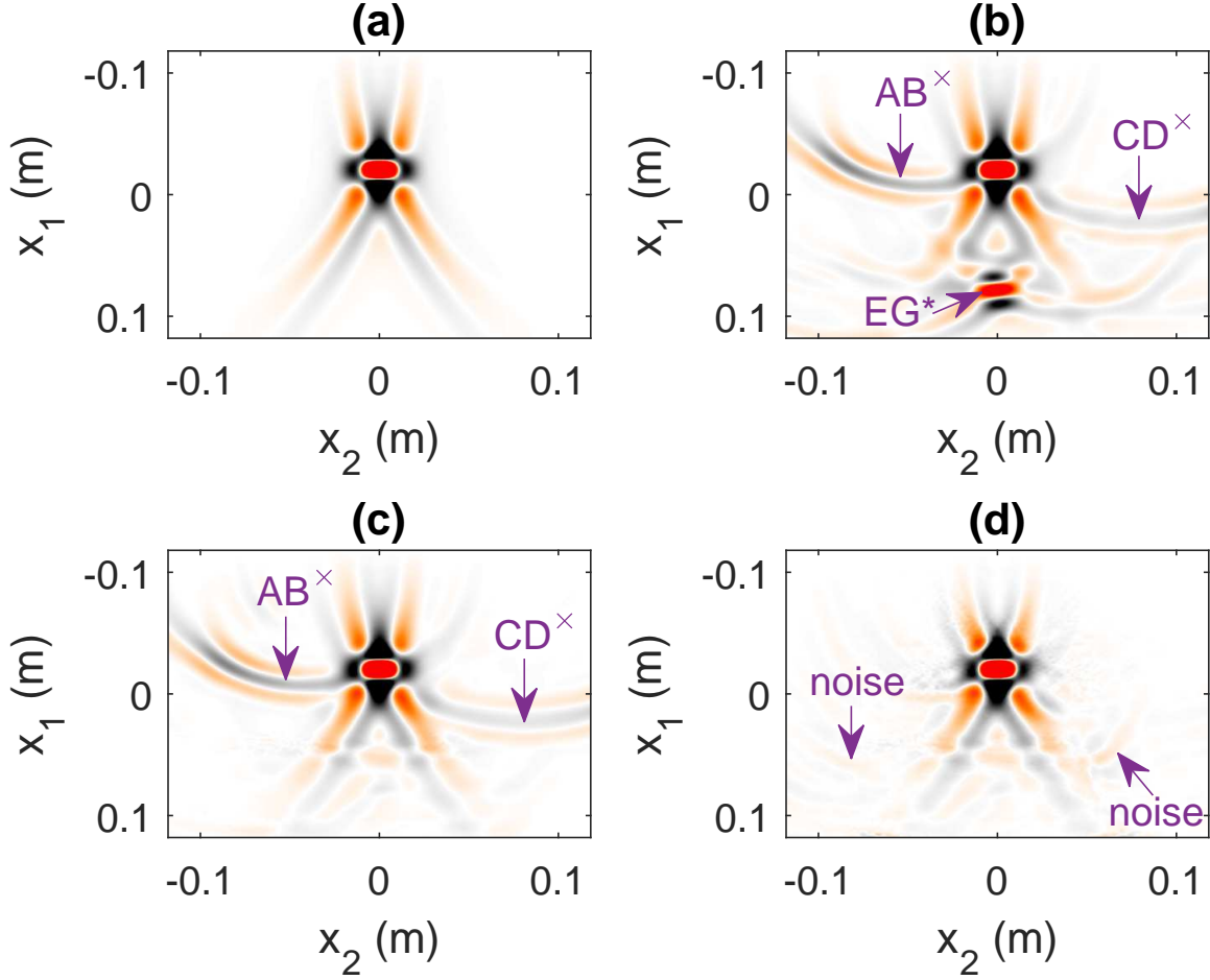
Fig. 12. Reconstructed initial pressure field \forall \mathbf{x} \in \mathbb{D} : p_e(\mathbf{x}, t = 0) . In panel (a) (which serves as a reference for the other panels), data have been computed in a homogeneous background medium and F_{Ud} acted as our focusing function. In panels (b)-(d), data have been computed in the heterogeneous medium of Fig. 3. (b) F_{Ud} acted as our focusing function. (c) The focusing function is obtained by solving the Marchenko equation under the direct-wave approximation F_{Ua} = 0 . (d) The focusing function is obtained by solving the auxiliary equation (with F_{Um} = 0 ) and the Marchenko equation successively. All panels are clipped at 10% of the maximum amplitude.
