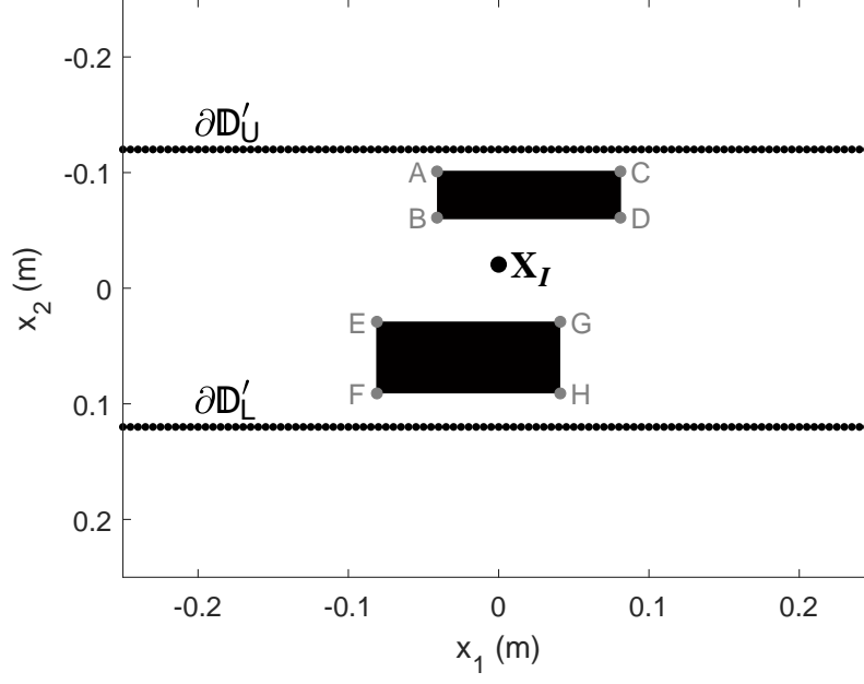
Fig. 3. Configuration for the 2D numerical experiment. The medium has a constant velocity of 1500\text{m/s} and a background density \rho_{white} = 1000\text{kg/m}^3 . The two black rectangles are density anomalies with \rho_{black} = 2000\text{kg/m}^3 . The gray dots (labeled as A, B, ..., H) denote sharp corners that generate forward-scattered waveforms. The upper boundary \partial\mathbb{D}'_U contains 101 coinciding vertical force (dipole) sources and pressure receivers with a spacing of 5\text{mm} . The lower boundary \partial\mathbb{D}'_L contains 101 vertical force (dipole) sources with a spacing of 5\text{mm} . Additional taper zones have been added to these arrays at the intervals x_1 \in [-0.5\text{m}, -0.25\text{m}) and x_1 \in (-0.25\text{m}, 0.5\text{m}] to eliminate truncation artefacts of the spatial integrals. The black dot marks the specific location \mathbf{x}_I = (0, -0.0205\text{m}) , where we retrieve our focusing function and Green's function.
