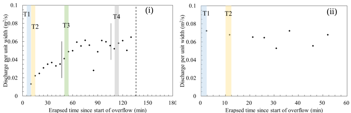
Figure 3. Time series of discharge per unit width and time intervals for numerical simulation of shear stress, \tau in each case (i) Clay case, (ii) Loam case
