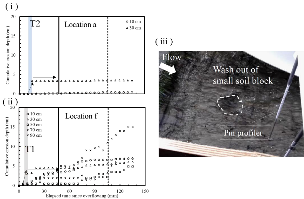
Figure 7. Erosion around points a and f for Clay.
