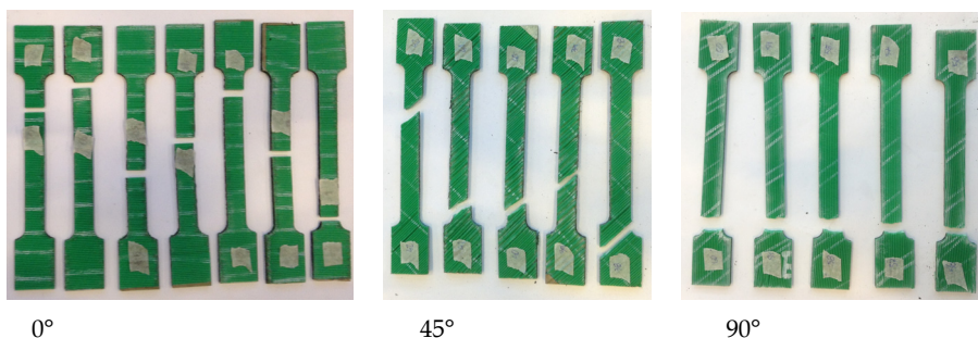
Figure 3: Tested specimens for the three print directions
