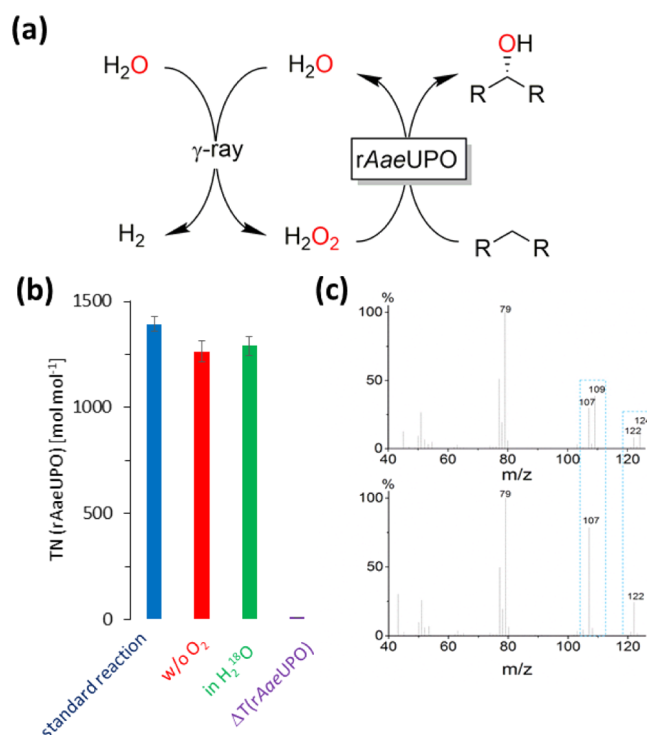
Figure 2. Selective hydroxylation of ethyl benzene to ( R )-1-phenyl ethanol using rAaeUPO and radiolysis-derived \text{H}_2\text{O}_2 : (a) reaction scheme; (b) turnover numbers ( \text{TN} = \text{moles}_{(\text{R})\text{-1-phenyl ethanol}} \times \text{moles}_{\text{rAaeUPO}}^{-1} ): (blue): standard reaction ( [\text{rAaeUPO}] = 200\text{ nM} , [\text{substrate}] = 5\text{ mM} ); (red): w/o \text{O}_2 (using deaerated reaction mixtures); (green): in \text{H}_2^{18}\text{O} (under aerobic conditions but using ^{18}\text{O} -enriched water); (violet): \Delta T(\text{rAaeUPO}) (using a thermally inactivated biocatalyst); (c) GC/MS analysis of the reaction product (( R )-1-phenyl ethanol) obtained from the reaction in ^{18}\text{O} -enriched water (upper) and under standard conditions (lower). Error bars indicate the standard deviation of duplicate experiments ( n = 2 ).
