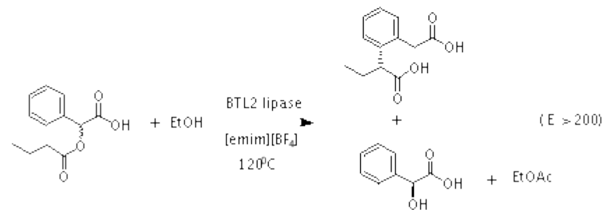
Figure 6. Lipase catalysed (trans)esterifications in ILs at 120°C
