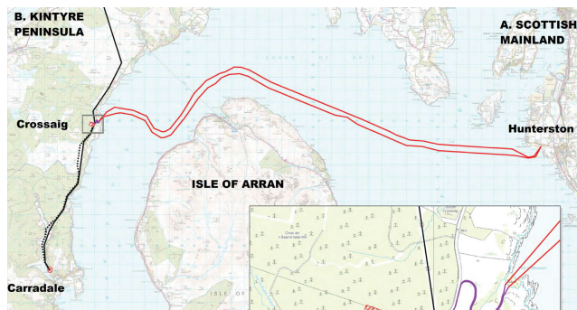
FIGURE 4. Hunterston-Kintyre project map [25].
