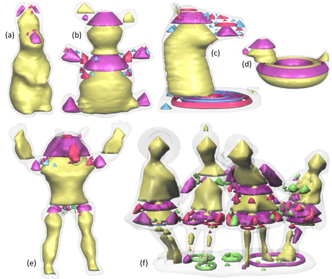
Fig. 17. More results generated by our support-free hollowing framework. Models with complex topology such as (f) can be well handled by our method. The different colors indicate the progressive results of repeated hollowing.
