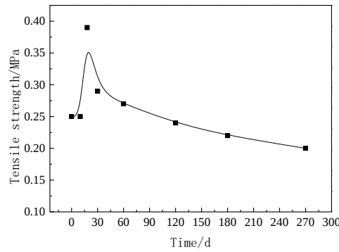
Fig. 3 Tensile strength in aging test (CARS)
