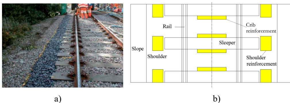
Fig. 15 Specific section bonding a) By P K Woodward, 2011, b) By Jing Guoqing, 2017
