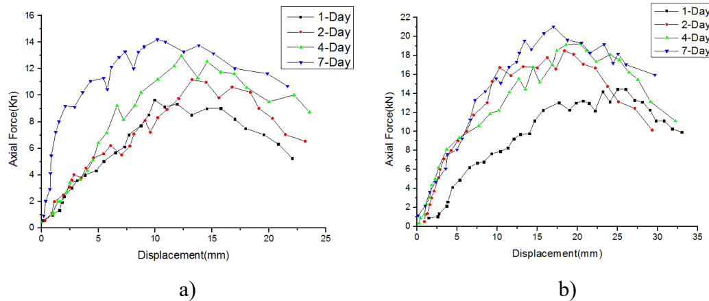
a) b) Fig.6 force-displacement curve of compression test a) 5.3Mpa polyurethane, b) 14.2Mpa polyurethane (Jing Guoqing, 2017)
