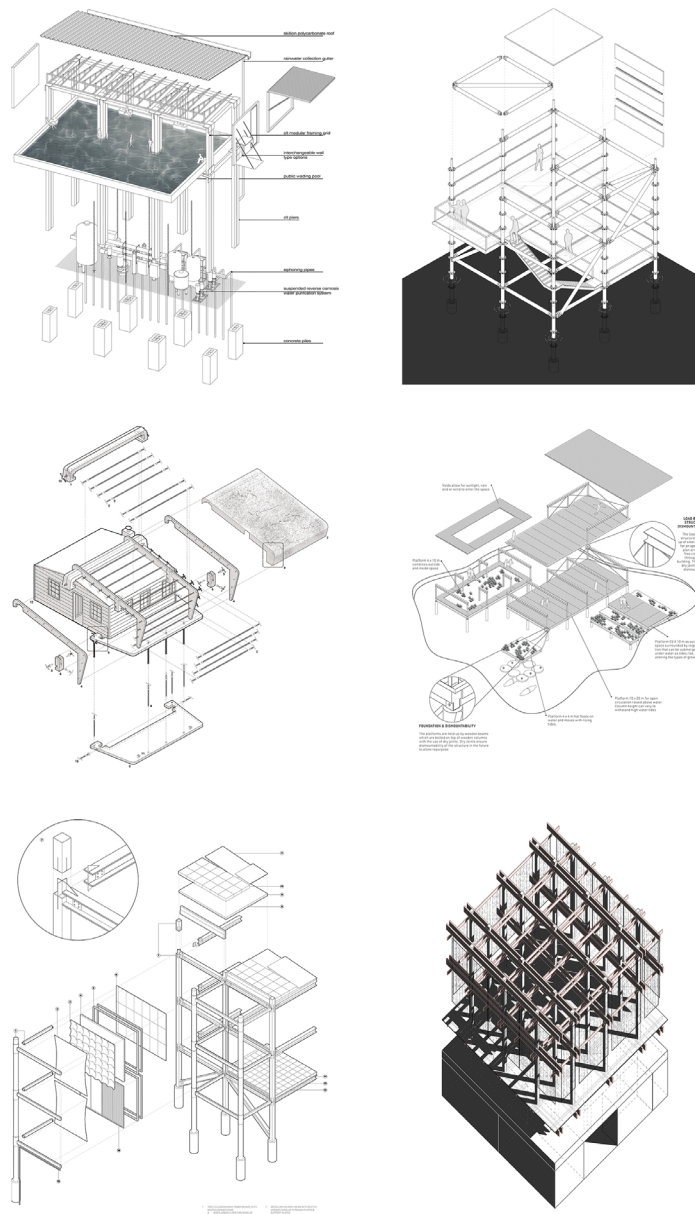
Figure 5. Resilient prototypes, axonometric projections (Camilla Casolari, William Chen, Lucas Jourdain, Lala Leung, Mary Perez, Isabel Roden. MSc. 2 Architectural Design Studio "Resilience-by-Design," 2024. Group of Public Building, Faculty of Architecture and the Built Environment, TU Delft. Instructors: Stefano Corbo, Sien van Dam)
