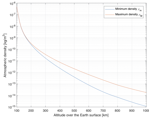
Figure 1.13: Atmospheric density with respect to altitude according to the Harris-Preister model. Based on table in [75, Ch.4].
