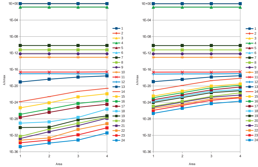
Figure 5.9: Variation of the eigenvalues with respect to spacecraft area for measurement case 1 (only relative position) at an altitude of 300 km. Left: with no initial rotation. Right: with initial rotation.
