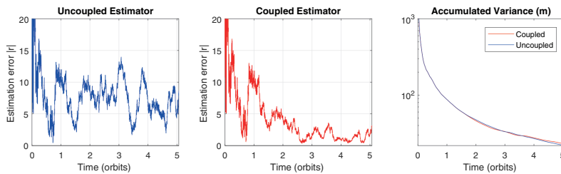
Figure 6.5: Variance of the error after five orbits at 650 km altitude.
