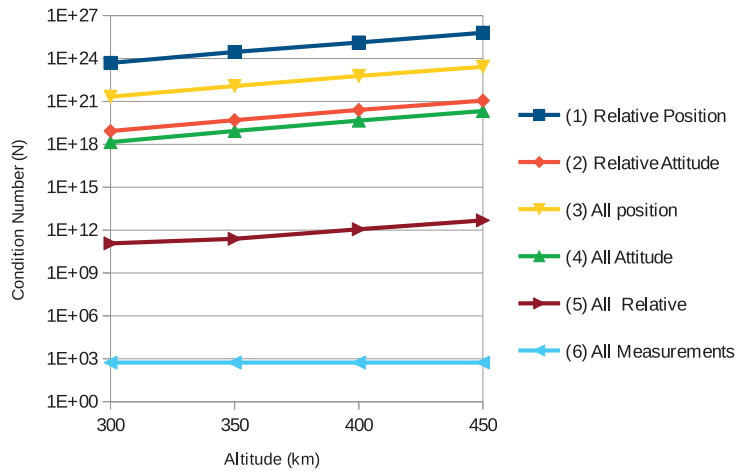
Figure 5.11: Observability degree vs to altitude for measurements described on Table 5.3
