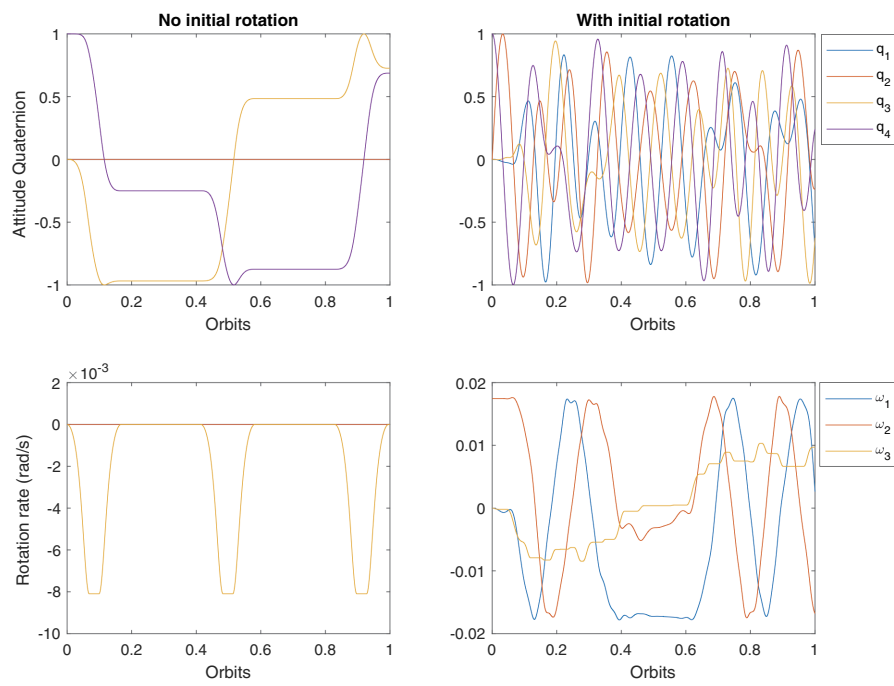
Figure 3.6: Propagation of attitude states over one orbit for the conditions given by Table 3.1.
