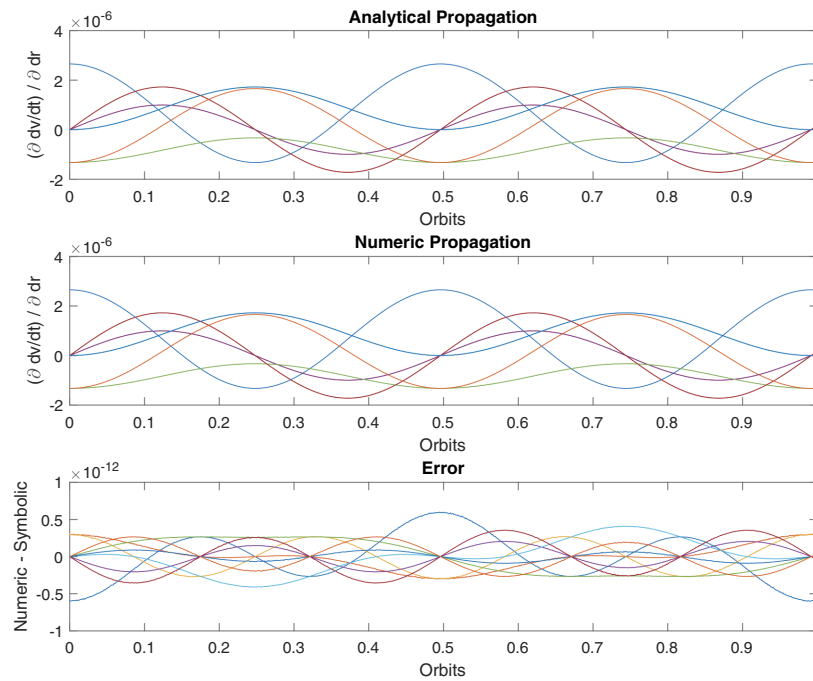
Figure 4.1: Propagation of the analytical and numeric partial derivative \partial \dot{\mathbf{v}} / \partial \mathbf{r} as an example of the verification
