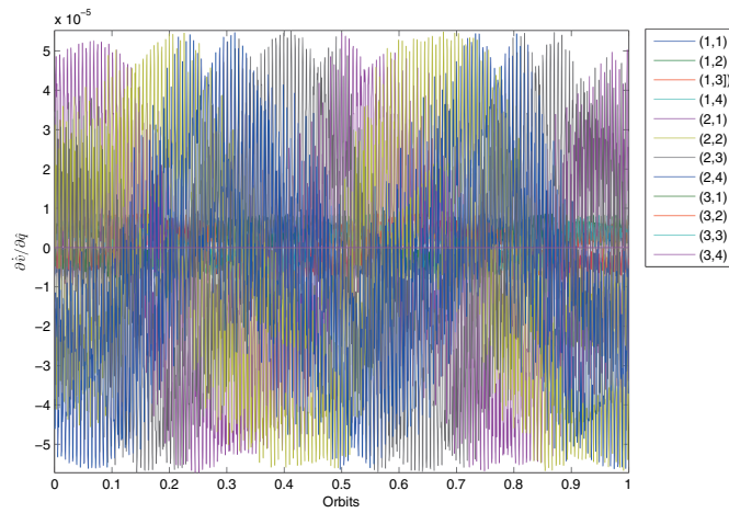
Figure 5.6: Variation of \partial \dot{\mathbf{v}} / \partial \dot{\mathbf{q}} when the system is initially rotating for one orbit on a spacecraft system with area configuration 1 (smallest).
