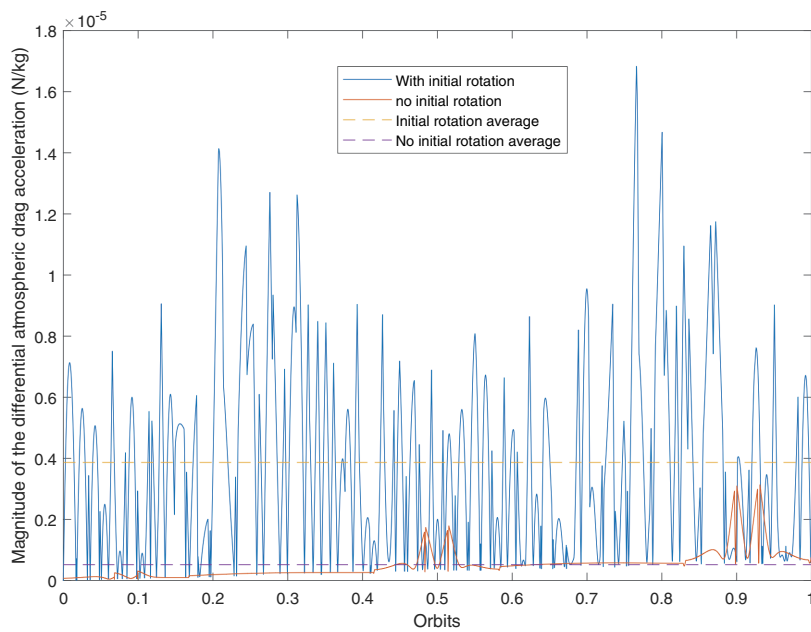
Figure 3.7: Propagation of the differential atmospheric drag acceleration over one orbit for the conditions given by Table 3.1.
