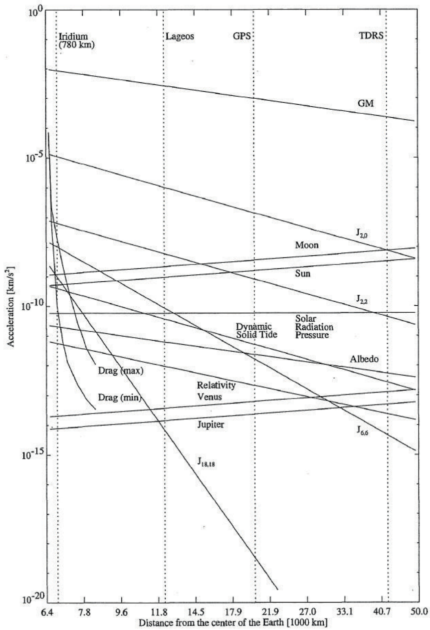
Figure 3.1: Order of magnitude of various perturbing accelerations of a satellite orbit [41].
