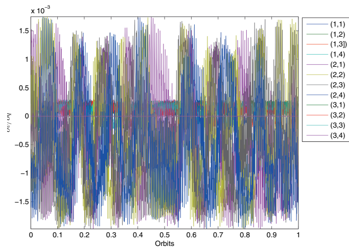
Figure 5.8: Variation of \partial \dot{\mathbf{v}} / \partial \mathbf{q} when the system is initially rotating for one orbit on a spacecraft system with area configuration 4 (largest)
