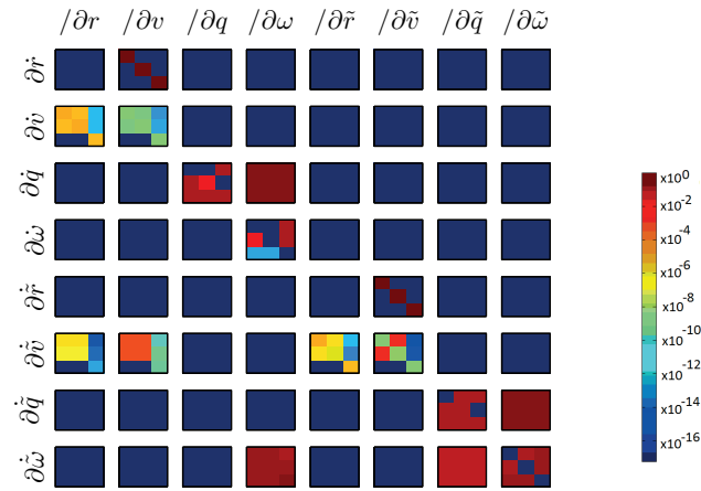
Figure 5.1: Maximum value of the gradient matrix of the space state system under study for case 1, area configuration 1, rotating, when coupling is not taken into account. Values are shown in a logarithm scale.
