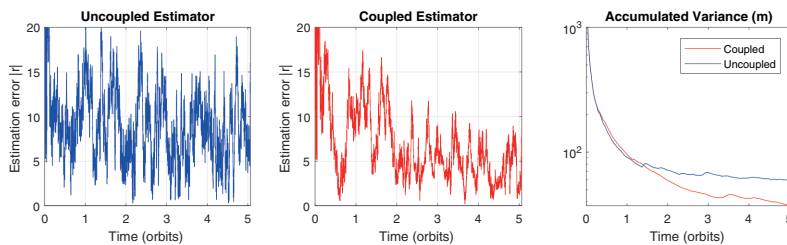
Figure 6.2: Relative position estimation results for the large spacecraft case.
