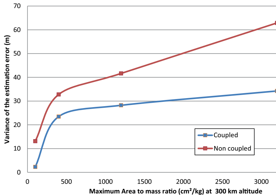
Figure 6.3: Variance of the error after five orbit with respect to the spacecraft area at a 300 km altitude.
