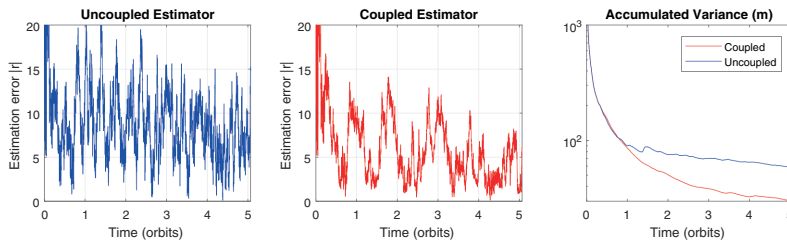
Figure 6.4: Variance of the error after five orbit at 350 km altitude.
