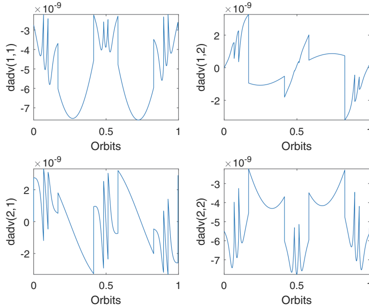
Figure 4.2: Propagation of the numerical variation of the atmospheric drag force with respect to the velocity. The derivation of the third component is not shown due to the fact that the propagation is done in an equatorial orbit.
