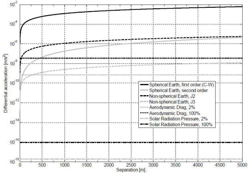
Figure 3.2: Order of magnitude of various differential perturbations for close near-circular formation as a function of spacecraft separation [100].
