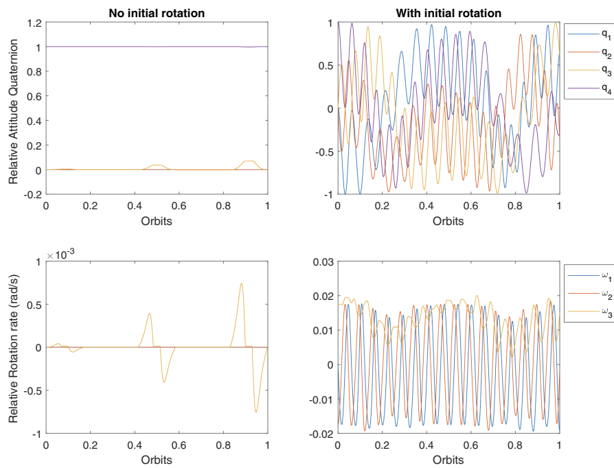
Figure 3.8: Propagation of the differential atmospheric drag acceleration over one orbit for the conditions given by Table 3.1.
