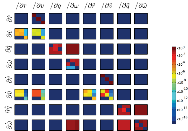
Figure 5.3: Maximum value of the gradient matrix of the space state system under study for case 1, area configuration 4, rotating, when coupling is not taken into account. Values are shown in a logarithm scale.
