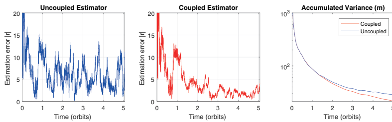
Figure 6.1: Relative position estimation results for a 2-spacecraft formation with 3-unit Cubesat configuration.
