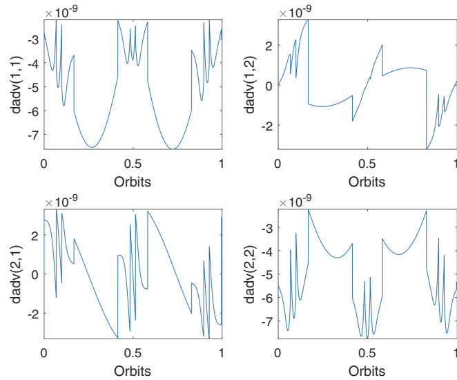
Figure 4.3: Propagation of the symbolic variation of the atmospheric drag force with respect to the velocity. The derivation of the third component is not shown due to the fact that the propagation is done in an equatorial orbit.
