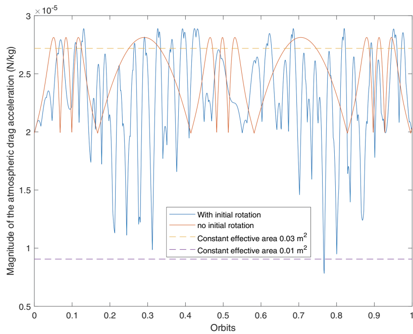
Figure 3.5: Propagation of the atmospheric drag acceleration over one orbit for the conditions given by Table 3.1.
