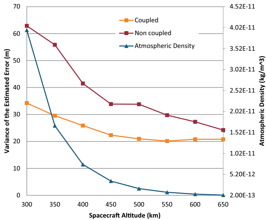
Figure 6.6: Variance of the error after five orbit with respect to the altitude.
