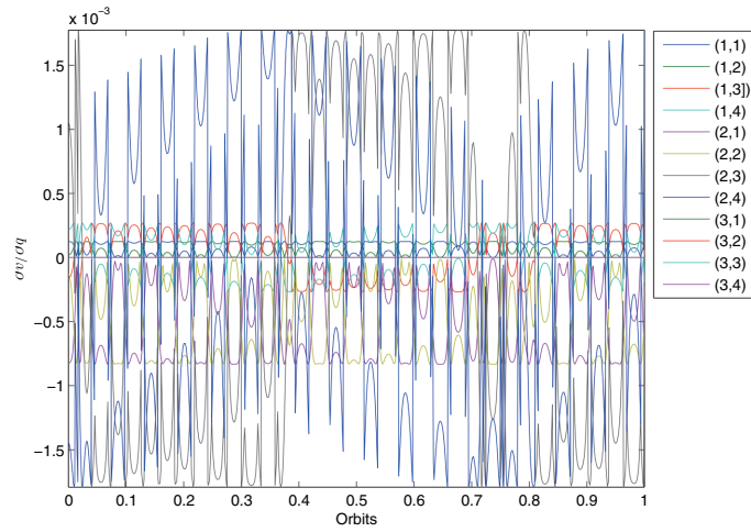
Figure 5.7: Variation of \partial \dot{\mathbf{v}} / \partial \mathbf{q} when the system is initially not rotating for one orbit on a spacecraft system with area configuration 4 (largest)
