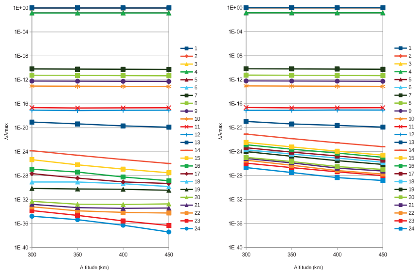
Figure 5.12: Eigenvalues variation vs altitude. Measurement case 1 (only relative position), Area Configuration 1 (30x10x10 cm). Left: with no initial rotation. Right: with initial rotation.
