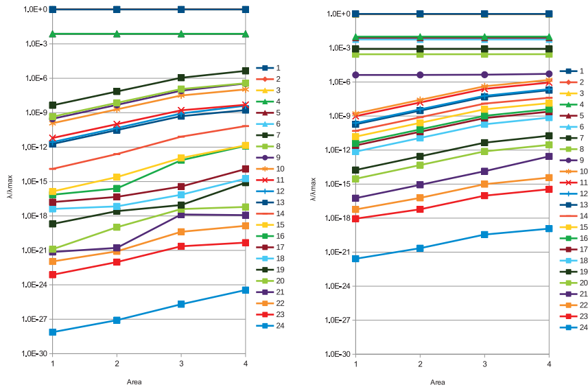
Figure 5.10: Variation of the eigenvalues with respect to spacecraft area. Measurement case 2 (only relative attitude) at an altitude of 300 km. Left: with no initial rotation. Right: with initial rotation.
