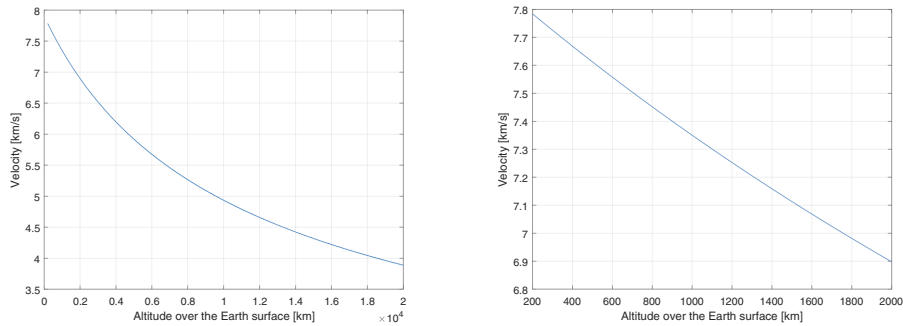
Figure 1.12: Orbital velocity with respect to altitude for a circular orbit from 200 to 20000 km (left) and from 200 to 2000 km (right).
