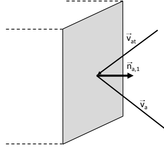
Figure 3.4: Representation of interaction of atmosphere particles with surface of a spacecraft. Specular reflection is assumed.
