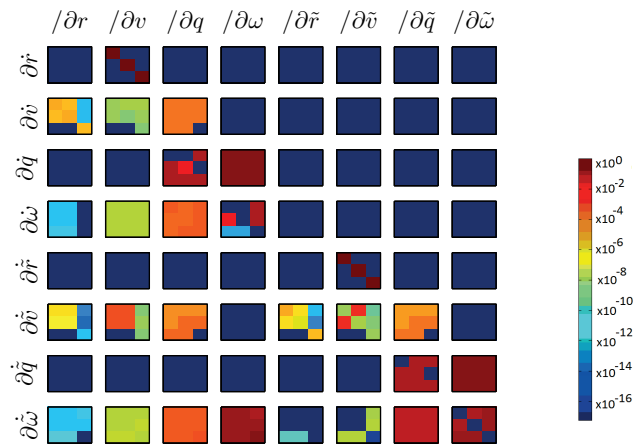
Figure 5.2: Maximum value of the gradient matrix of the space state system under study for case 1, area configuration 1, rotating when coupling is taken into account. Values are shown in a logarithm scale.
