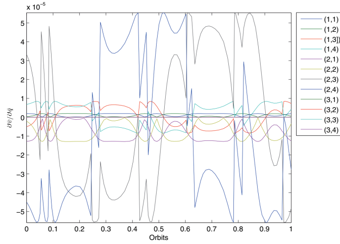
Figure 5.5: Variation of \partial \dot{\mathbf{v}} / \partial \dot{\mathbf{q}} when the system is not initially rotating for one orbit on a spacecraft system with area configuration 1 (smallest)
