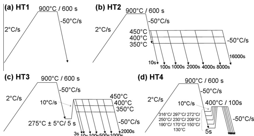
Fig. 2. Heat treatments applied to the steel: (a) HT1 to establish the required quenching rate; (b) HT2 to investigate bainite formation; (c) HT3 to investigate the dependence on partitioning conditions; (d) HT4 to investigate the dependence on quenching temperature.
