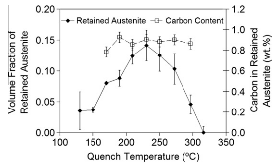
Fig. 8. Volume fraction of retained austenite and corresponding carbon content after full austenitization, quenching to different temperatures and partitioning at 400 \text{ }^{\circ}\text{C} for 100 s (heat treatment HT4).
