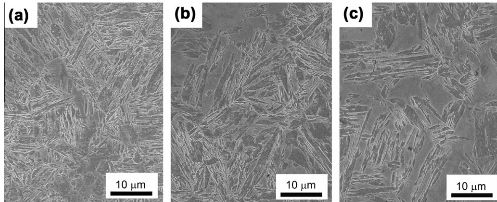
Fig. 6. Scanning electron micrographs of the steel after full austenitization, quenching to 275 \pm 5 \text{ }^{\circ}\text{C} and partitioning for 1000 s at: (a) 350 \text{ }^{\circ}\text{C} , (b) 400 \text{ }^{\circ}\text{C} , and (c) 450 \text{ }^{\circ}\text{C} . The specimens were etched with 2% nital.
