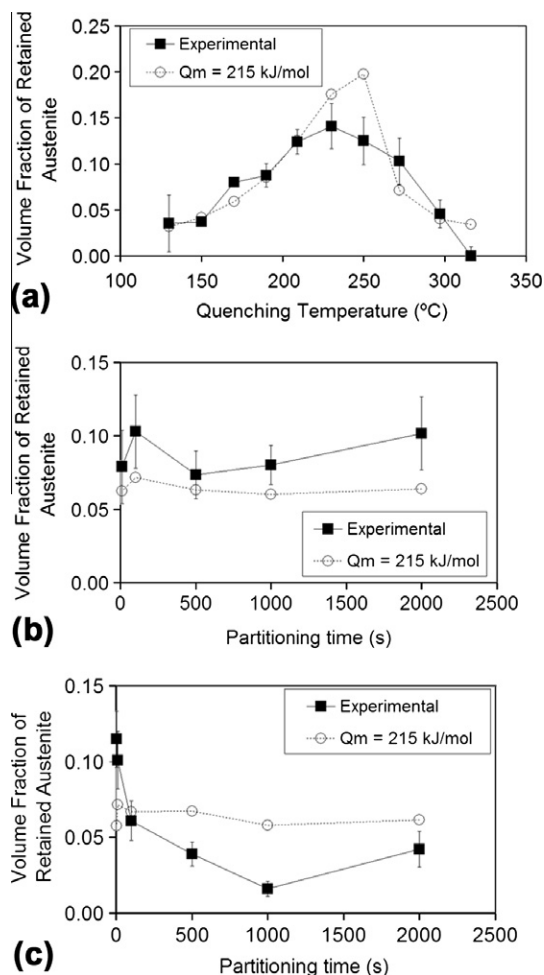
Fig. 11. Comparison between experimental and calculated values of volume fractions of retained austenite: (a) treatment HT4; (b and c) treatment HT3 with partitioning at (b) 400 °C and (c) 450 °C.
