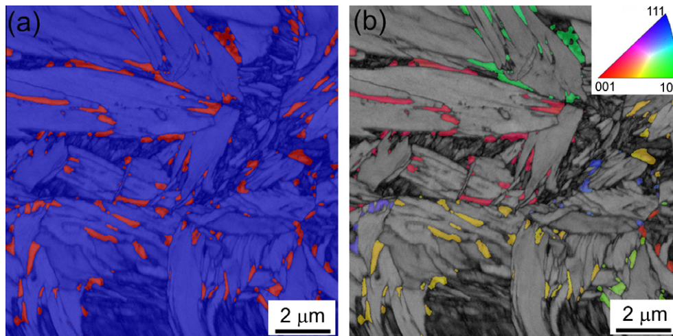
Fig. 7. EBSD analysis of the microstructure obtained after full austenitization, quenching to 275 \pm 5 \text{ }^{\circ}\text{C} and partitioning at 450 \text{ }^{\circ}\text{C} for 10 s.
