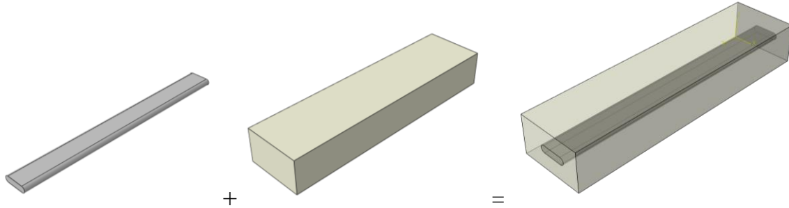
Figure 4: Overview of adding the carbon fibre geometric representation on the left to the nylon ‘host’ material in the middle. The result is a combined material using independent meshes.
