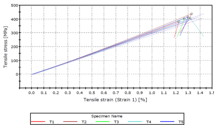
Figure 8: Results of the tensile tests for five coupons and test setup on the right
