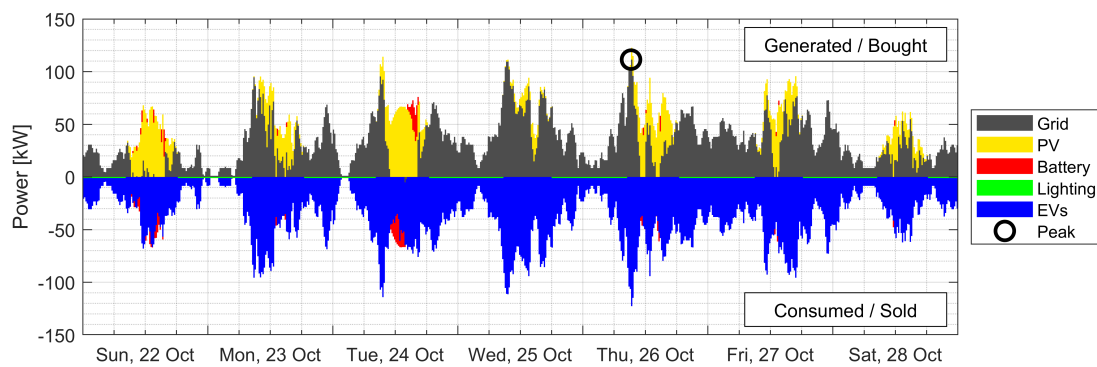
(a) Energy flows (unscheduled charging).
