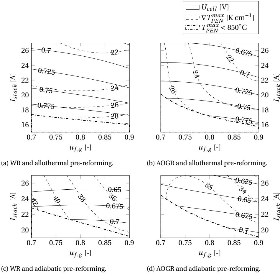
Figure 6.7: Cell voltages and maximum PEN temperature gradients in the stack for different reforming configurations, fuel utilisations and stack currents.
