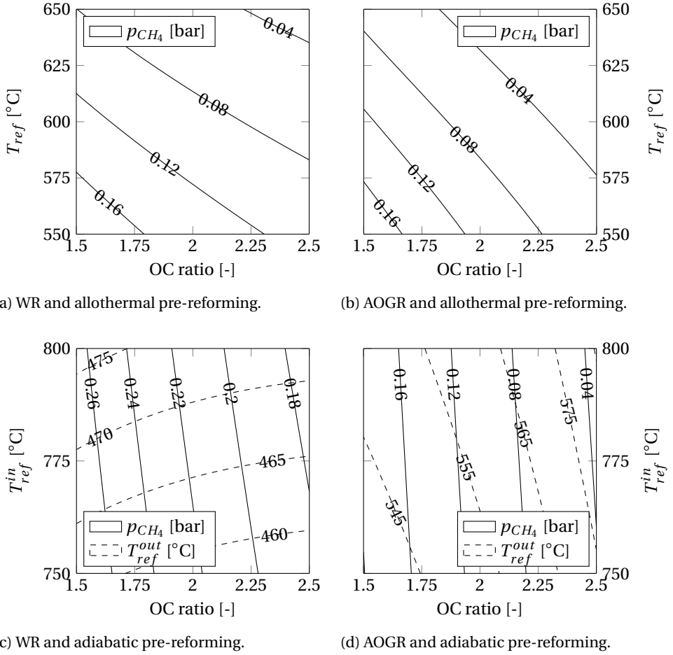
Figure 6.4: Methane partial pressures and outlet temperatures of adiabatic reformers for different reforming configurations, OC ratios and reformer (inlet) temperatures.
