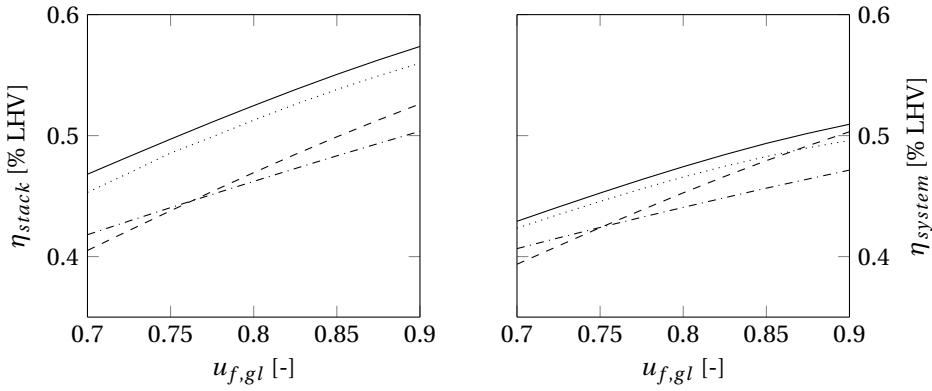
(c) Stack efficiency.
