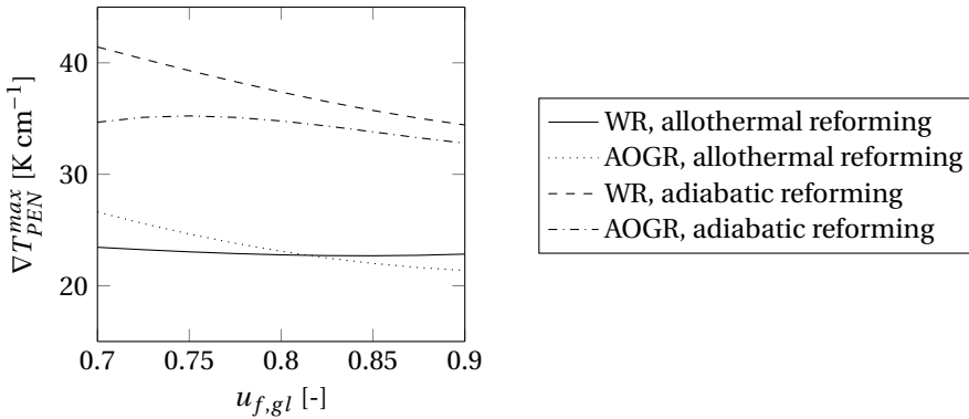
(e) Maximum PEN temperature gradient.
