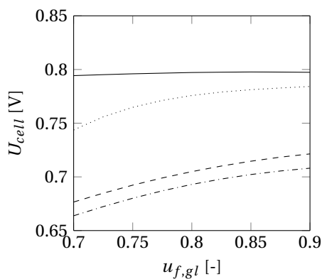
(a) Cell voltage.
