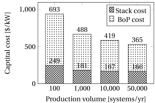
(c) 250 kWe SOFC CHP system.
