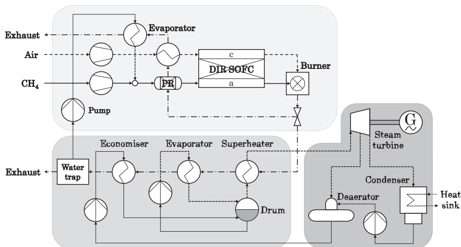
(d) SOFC-steam turbine combined cycle with isothermal pre-reforming and WR.
