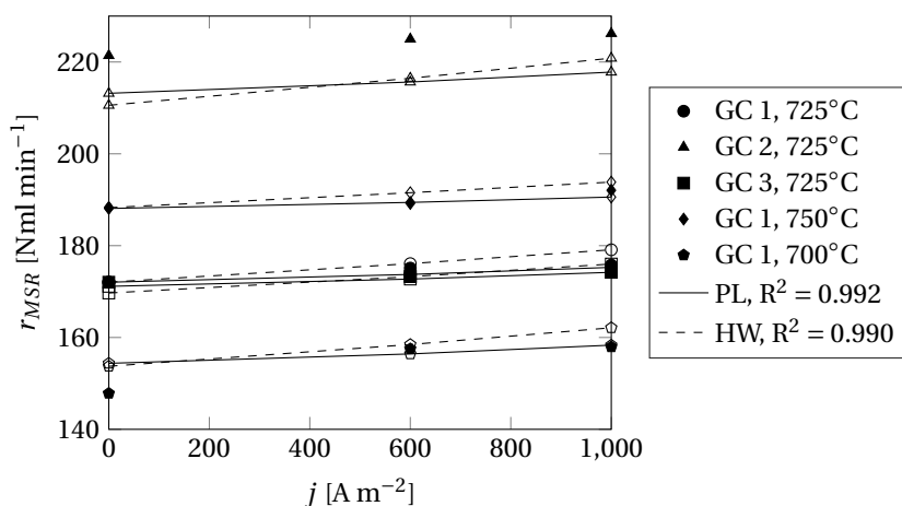
Figure 4.8: Overall methane steam reforming rates predicted with the 1D single cell model with PL and HW kinetics ( \circ \triangle \square \diamond \square ) versus the experimental values ( \bullet \blacktriangle \blacksquare \blacklozenge \bullet ) for various gas compositions, temperatures and electrochemical current densities.
