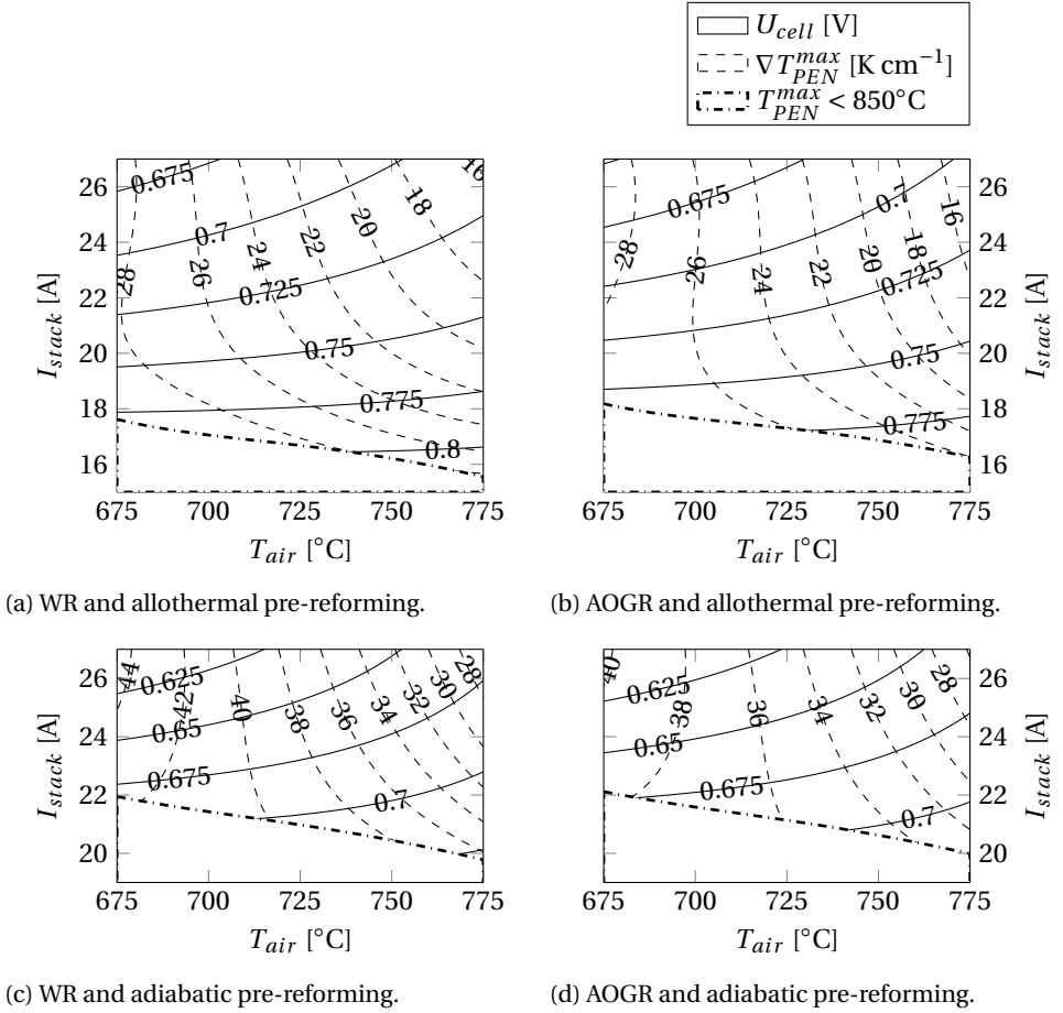
Figure A.3: Cell voltages and maximum PEN temperature gradients in the stack for different reforming configurations, cathode air inlet temperatures and stack currents.
