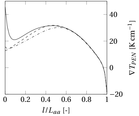
(c) PEN temperature gradients.
