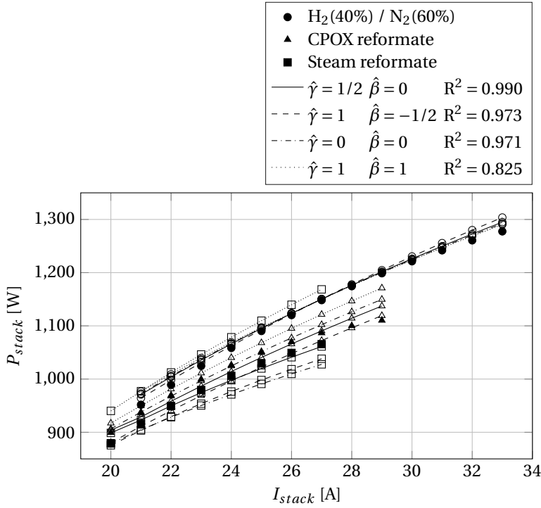
Figure 4.3: Simulated power curves for \text{H}_2/\text{N}_2 (○), CPOX (△) and SR (□) fuel versus data provided by Sun-fire/Staxera for their ISM V3.3 (●▲■) for different global reaction orders for hydrogen ( \hat{\gamma} ) and steam ( \hat{\beta} ) in the anode exchange current density.
