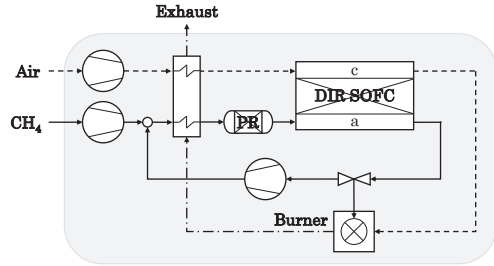
(a) Stand-alone reference SOFC system.
