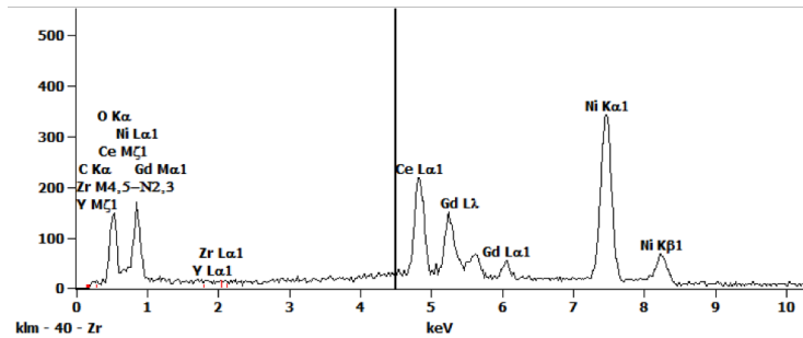
(b) EDX analysis after experiment.
