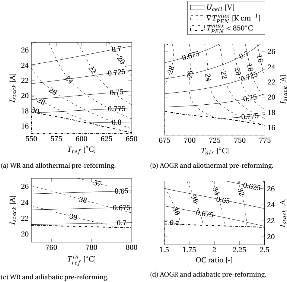
Figure 6.8: Cell voltages and maximum PEN temperature gradients in the stack for different reforming configurations and changes in the allothermal pre-reformer temperature (Figure 6.8a) and adiabatic pre-reformer inlet temperature (Figure 6.8c) for WR and various cathode air inlet temperatures (Figure 6.8b) and OC ratios (Figure 6.8d) for AOGR.
