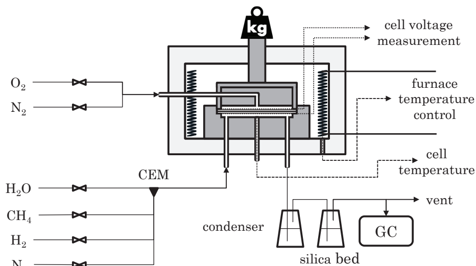
Figure 5.1: Schematic overview of the experimental single cell setup.
