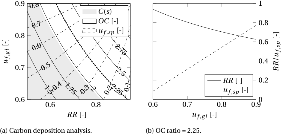
Figure 3.2: Carbon prone region for temperatures \leq 575^\circ\text{C} and contours of the OC and single pass fuel utilisation for various global fuel utilisations and anode off-gas recirculation ratios (Figure 5.3), and recirculation ratio and single pass fuel utilisation as a function of global fuel utilisation at OC ratio = 2.25 (Figure 3.2b)
