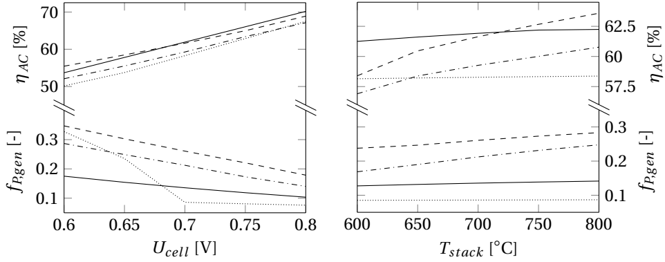
(b) \max(\eta_{AC}) , T_{stack} = 700^{\circ}C and \Pi_{comp} = 4 . (c) \max(\eta_{AC}) , U_{cell} = 0.7V and \Pi_{comp} = 4 .
