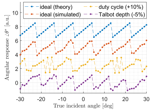
Fig. 3. Angular response \angle\theta^* as a result of simulation of the ASPs considering different effects. The individual ASP simulation results are combined through (4). The curves are shifted to improve readability.
