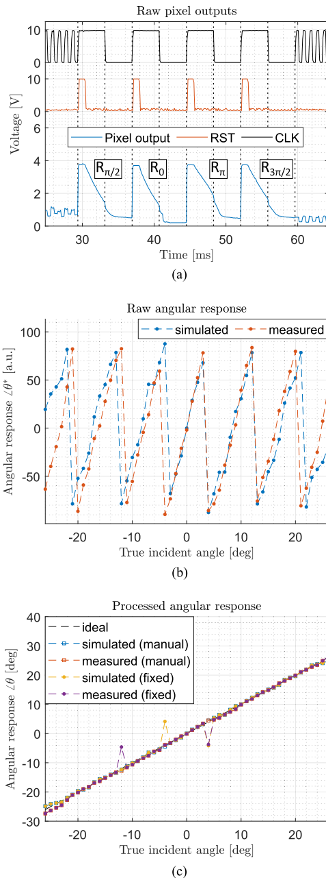
Fig. 6. Measurement results of (a) raw pixel outputs for a fixed incident angle. The fast CLK before and after the pixels of interest quickly cycles through the 64-pixel array. Derived (b) angular response using the extracted slope of each pixel [see (4)] and (c) processed response by manually identified or fixed angular periods [see (5)].
