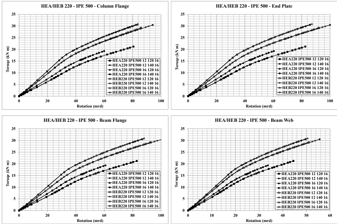
Fig.15: Moment vs. rotation curves for the fourth block:
