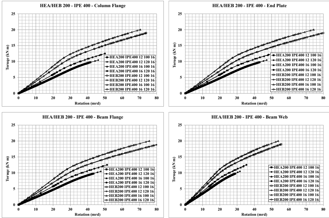
Fig.14: Moment vs. rotation curves for the third block:
