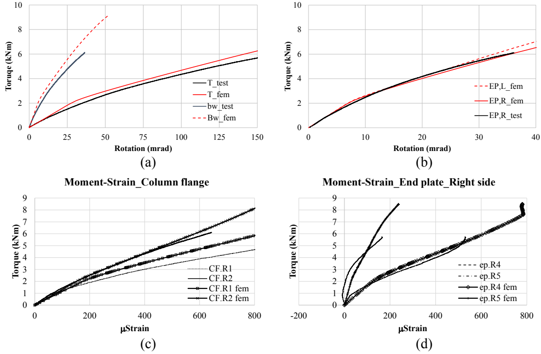
Fig. 9: Comparisons between test TT02 and FEM
