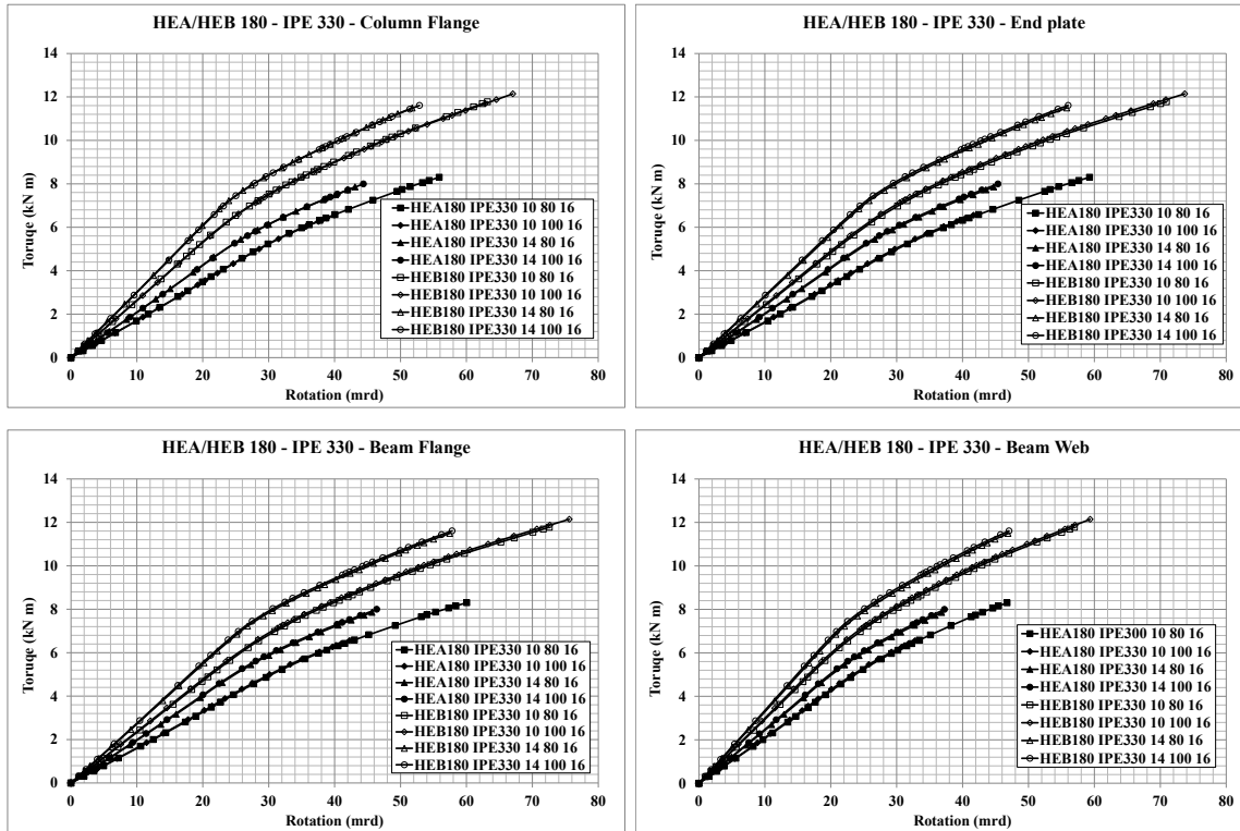
Fig.13: Moment vs. rotation curves for the second block:
