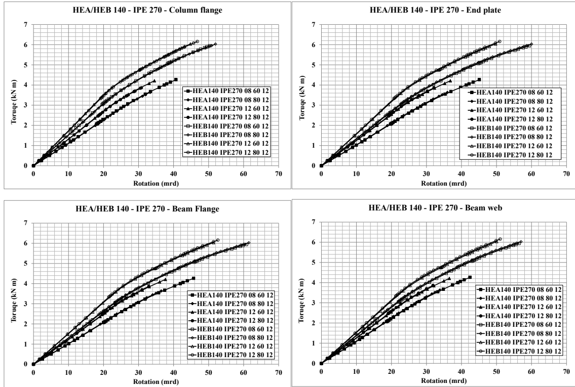
Fig.12: Moment vs. rotation curves for the first block:
