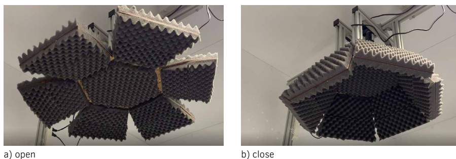
FIG. 8.4 The prototype of the individually controlled noise-reducing device.
