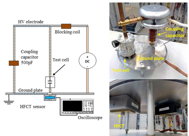
Fig. 1. PD measuring setup of surface discharges in SF 6 under DC voltage.
