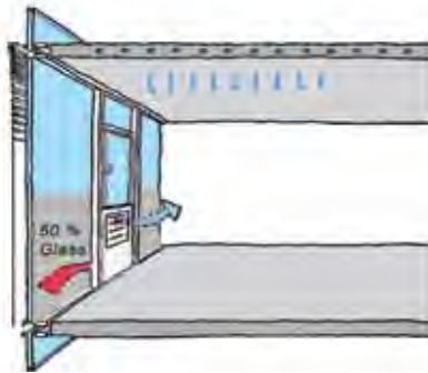
Figure 6.27 System recommendations cooling, London
