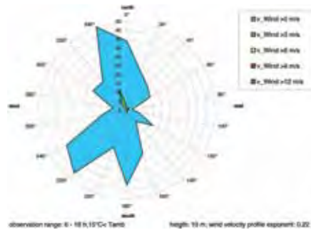
Figure 2.77 Wind rose, Moscow, day time above 15°C
