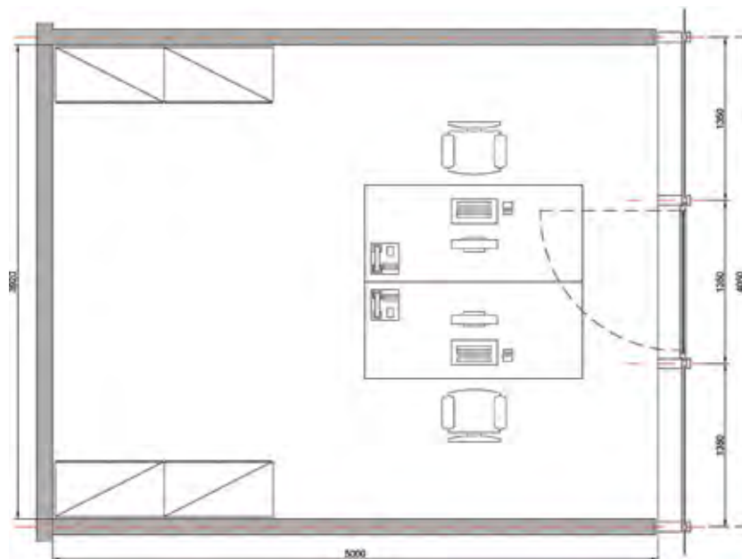
Figure 6.44 Floor plan of the test room configurations
