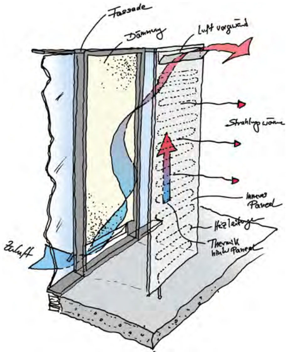
Figure 7.7 Conceptual sketch
