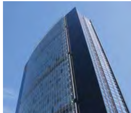
Figure 4.7: ARAG Duesseldorf, Foster and Partner with RKW, 2000 Shaft-box façade: The gap is minimised and designed such that supply air streams in across individual storeys whereas exhaust air is heated in a shaft within the façade and thus rises upward.
