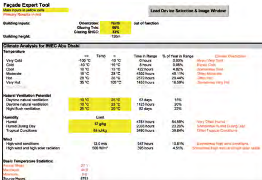
Figure 6.17 FET Climate analysis, Abu Dhabi
