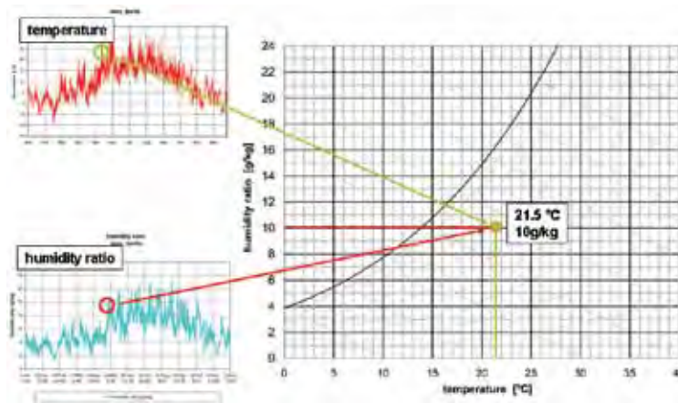
Figure 2.7 Summary of the temperature and humidity measurements in a psychrometric chart
