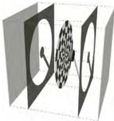
Figure 7.23: Construction Design principle ( L. van Ginkel )
