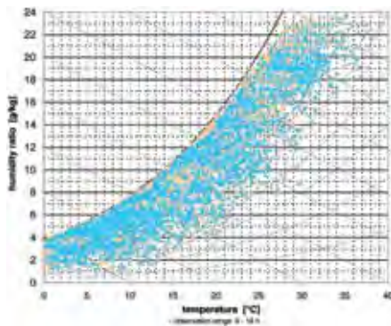
Figure 2.121: Psychrometric chart Shanghai
