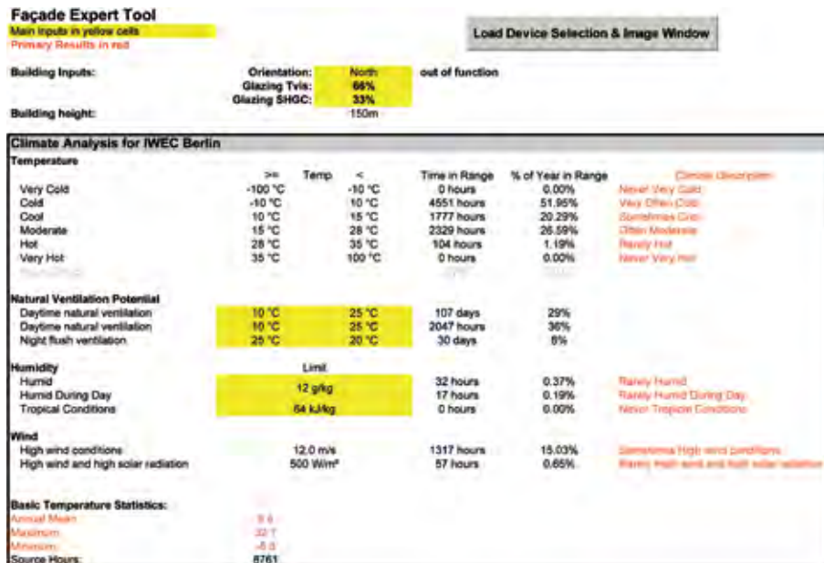
Figure 6.20 FET Climate analysis, Berlin
