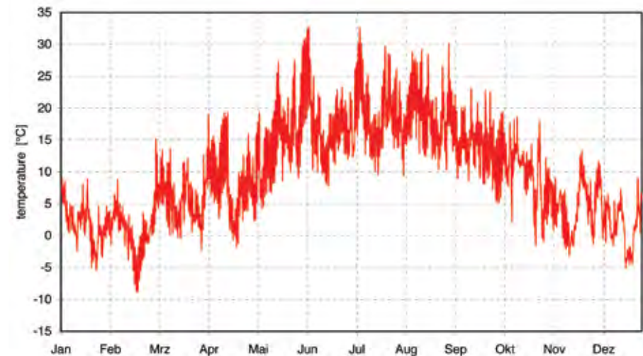
Figure 2.3 Annual temperature profile for Berlin, Germany
