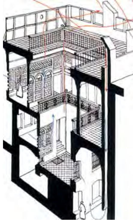
Figure 3.26: Convection ventilation in a courtyard.
