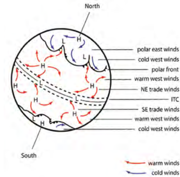
Figure 2.12 Primary wind and pressure system (Dahl)
