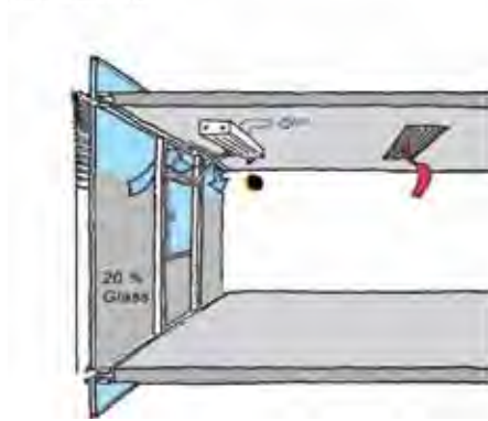
Figure 6.33 System recommendations cooling, New York
