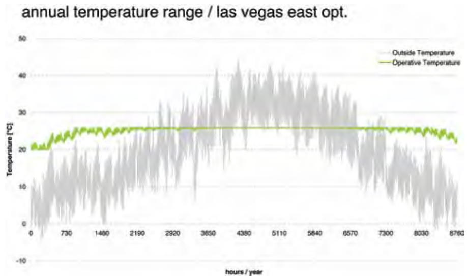
Figure 6.53 Annual temperature profile in the optimised test room including interior and exterior temperatures, Eastern Las Vegas
