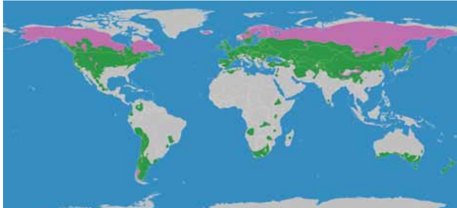
Figure 3.3 Expansion of the boreal or snow-forest climate moderate zone pink: cold moderate borealis climate green: warm moderate climate
