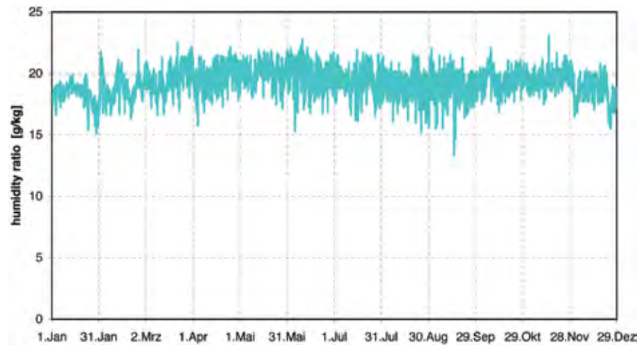
Figure 2.107 Annual air humidity profile, Singapore
