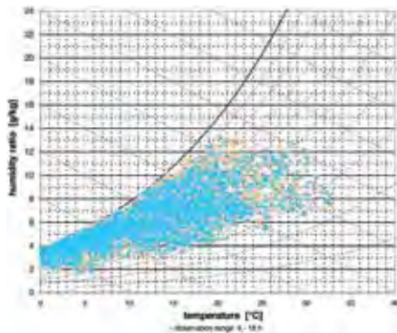
Figure 2.115: Psychrometric chart Berlin
