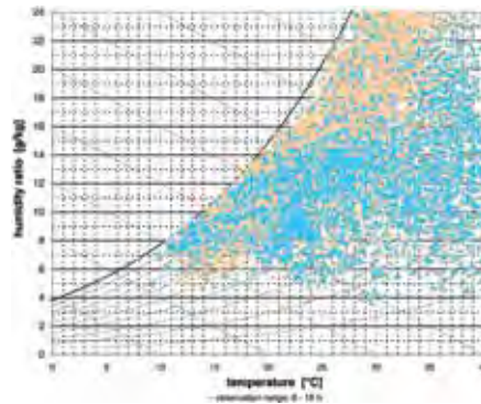
Figure 2.116: Psychrometric chart Abu Dhabi
