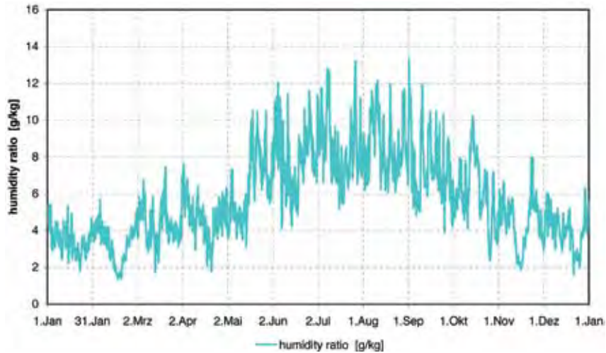
Figure 2.23 Annual air humidity profile, Berlin
