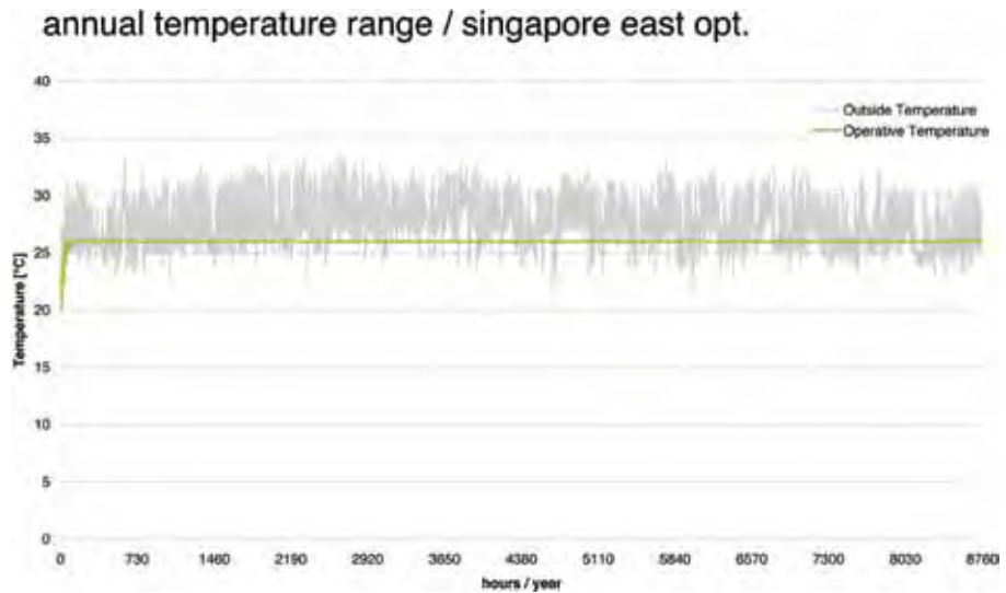
Figure 6.73 Annual temperature profile in the optimised test room including interior and exterior temperatures, Eastern Singapore
