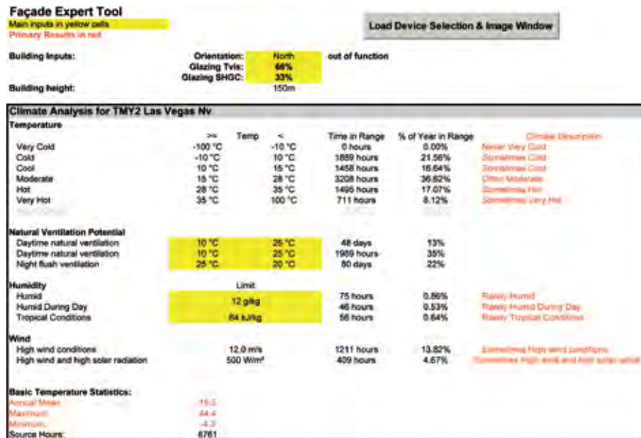
Figure 6.23 FET Climate analysis, Las Vegas
