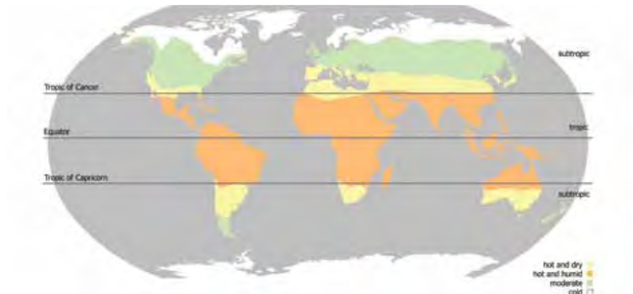
Figure 2.2 Extremely simplified climate zone classification
