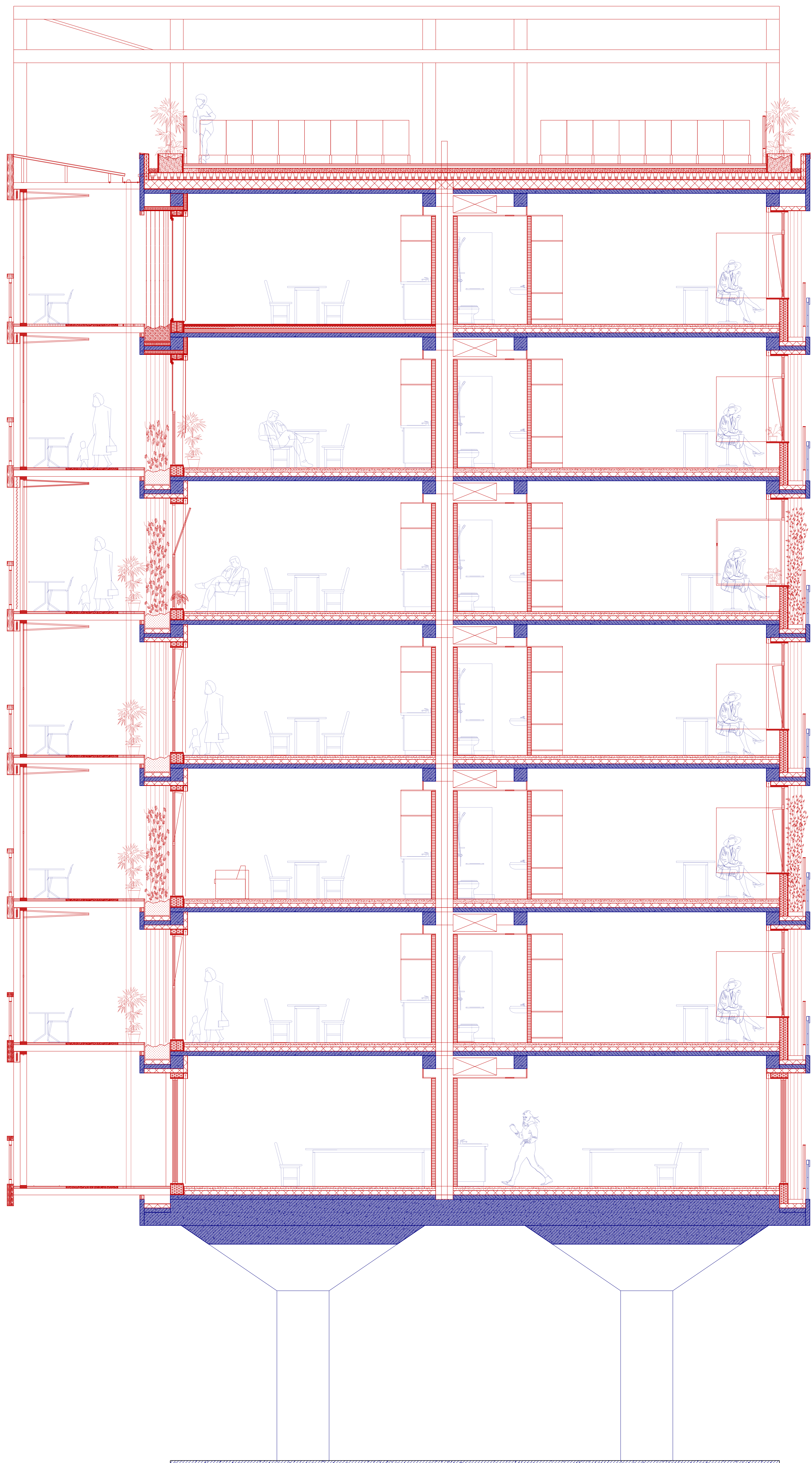
Section 1: 50
