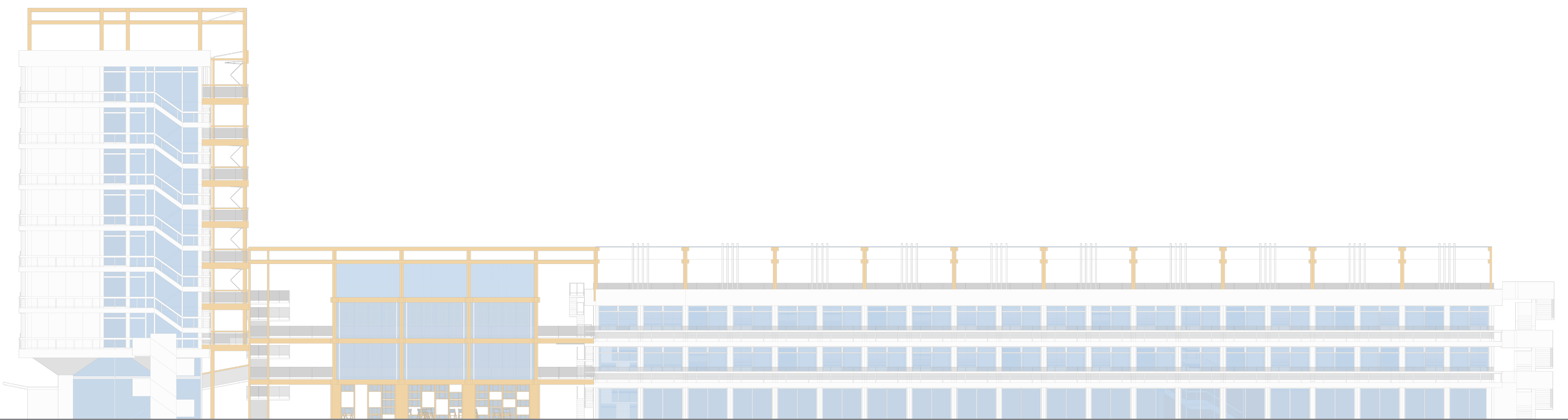
East Elevation 1:250
