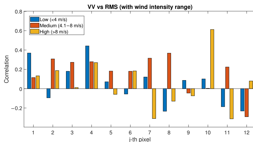
Figure 16. Correlation factor between SAR (VV polarisation) and RMSH evaluated for low-, medium- and high-wind-speed conditions.
