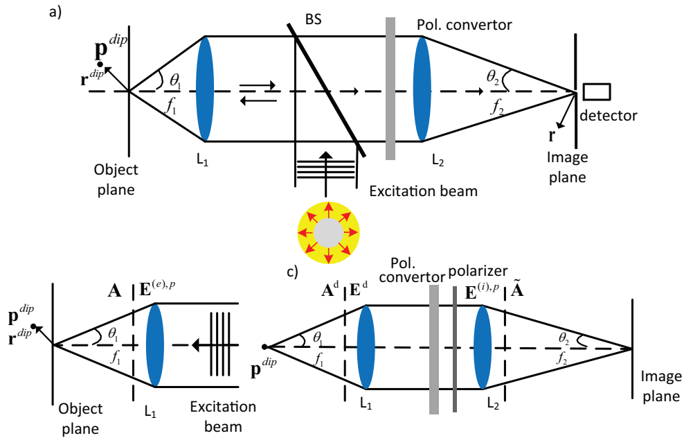
Fig. 1. Schematic of the confocal microscope. A beam splitter divides the excitation path and detection path into two arms. A laser beam is focused onto the sample by a high NA objective lens L_1 . The light scattered by the sample is collected by the same objective lens and focused by a small NA lens onto a pinhole in front of a detector. a) The complete confocal microscopy system, b) Focusing and dipole excitation, c) Imaging and polarization conversion.
