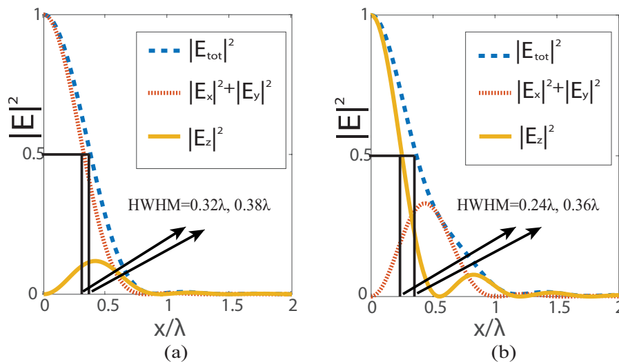
Fig. 2. Profiles of the squared amplitude of the longitudinal and transverse components and total energy density |\vec{E}|^2 in the focal plane in the case of a pupil field that is linearly polarized in the x - direction (a) and a pupil field that is radially polarized (b). The focusing lens has NA=0.9. The plots are normalized to the on-axis peak values.
