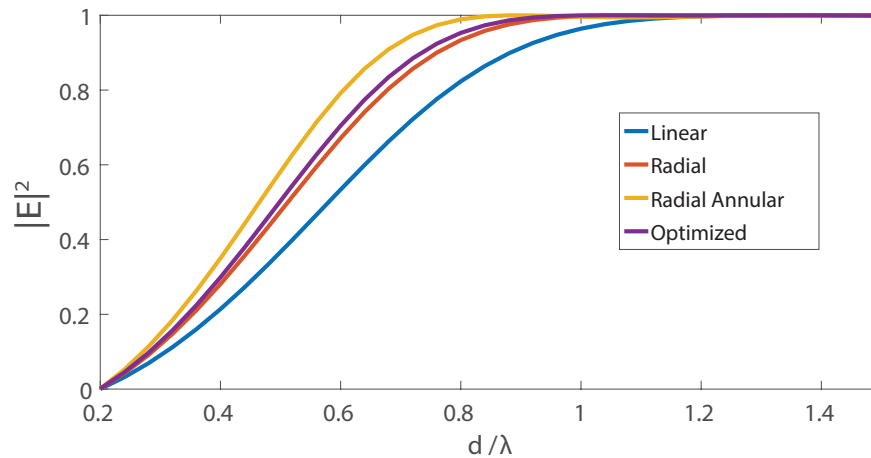
Fig. 6. Profiles of the visibility as a function of the d/\lambda for the four cases of pupil fields. The system is the same as shown in Fig. 5.
