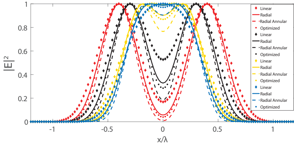
Fig. 5. Profiles of the detected intensities as function of scanning distance of two separated dipoles for different kinds of illumination and for several distances between the dipoles. The system is composed of two lenses with NA_1 = 0.9 , and NA_2 = 0.3 and is illuminated by light with a wavelength of \lambda = 500nm . The illumination is either linearly, radially or optimized radially polarized. The two dipoles are set along the x axis for the linear polarization and along the z axis for the other radially polarized cases. A polarization converter is added in the case of radially polarized excitation. Four different distances between the dipoles are chosen: d=0.8\lambda (red line), d=0.6\lambda (black line), d=0.4\lambda (yellow line), and d=0.36\lambda (blue line). The plots are normalized to the on-axis peak intensity.
