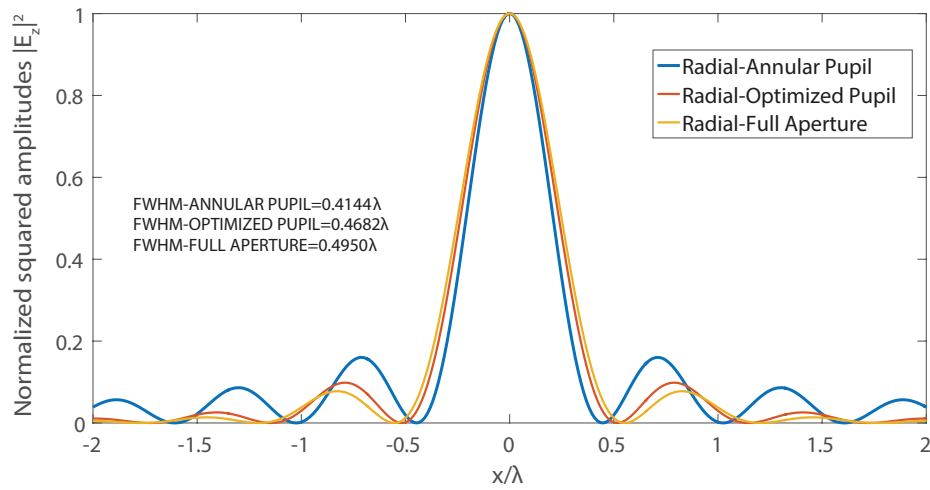
Fig. 3. Profiles of the squared amplitudes of the longitudinal components of the exciting spot in the focal plane in the case of radially polarized illumination with full aperture, annular aperture and optimized radially polarized pupil field. The plots are normalized to their on-axis maxima.
