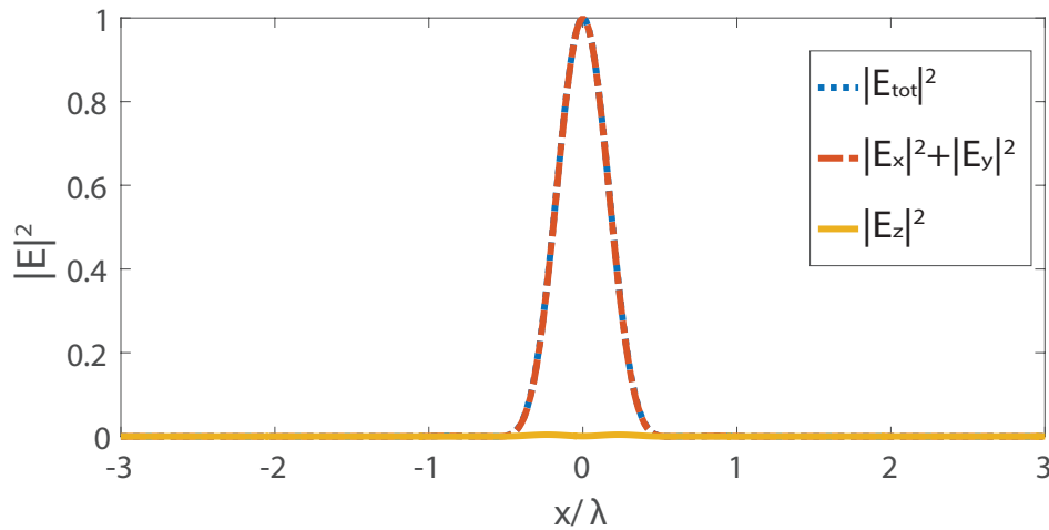
Fig. 4. Profiles of the intensities at the detector plane with a polarization convertor and a small pinhole with radius r = 0.18 \mu\text{m} which is 0.36\lambda in terms of wavelength. The system is composed of: a high \text{NA}_1 = 0.9 focusing objective lens and a low \text{NA}_2 = 0.3 lens for detection. For illumination, radially polarized light of wavelength \lambda = 500\text{nm} is used. The focal field can be seen in Eq. (17). The dipole is set rigidly along the z -axis direction (only \alpha_{zz} is relevant). The plots are normalized to on-axis maxima.
